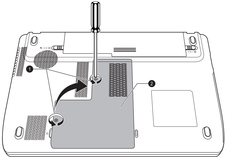
Figure 3-9 Removing the memory module cover
