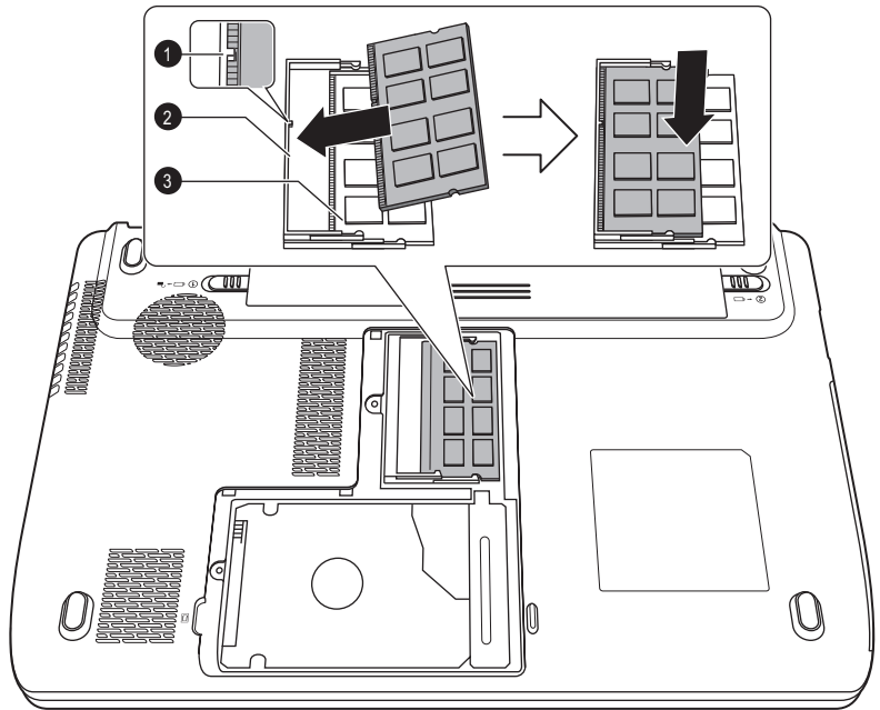
Figure 3-10 Seating the memory module
