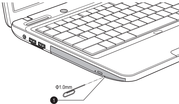
Figure 3-5 Manual release with the eject hole
