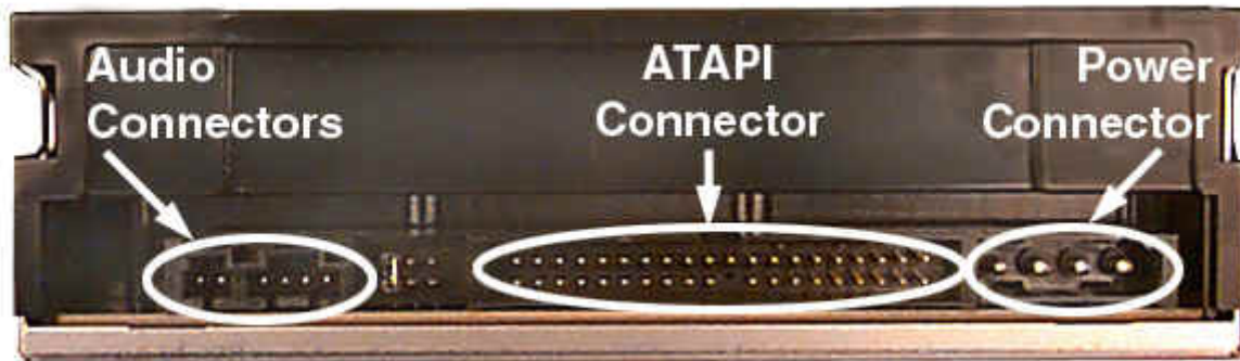
Figure 1. SD-M1502 DVD-ROM Drive Rear Panel - Connectors
