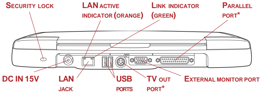
Figure 2-4 The back side of the computer
