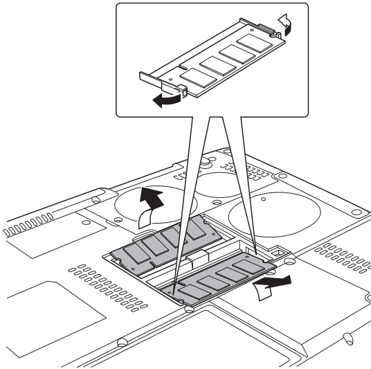
Figure 8-5 Removing the memory module
