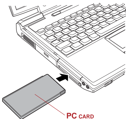
Figure 8-1 Installing the PC card
