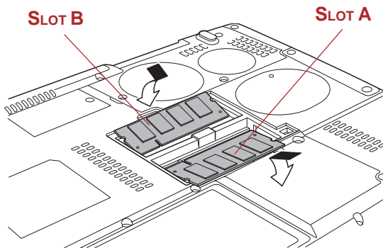
Figure 8-4 Installing the memory module
