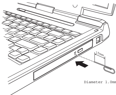
Figure 4-4 Manual release with the eject hole
