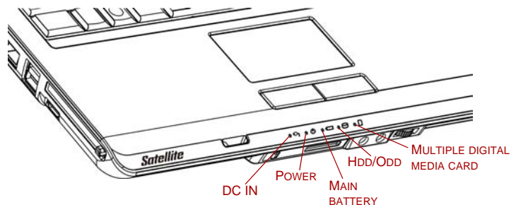
Figure 2-7 System indicators
