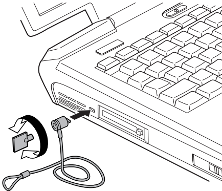
Figure 8-16 Security lock
