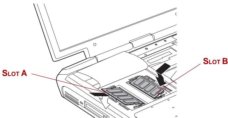
Figure 8-11 Installing two memory modules
