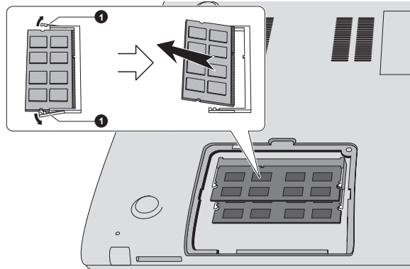
Figure 4-9 Removing the memory module
