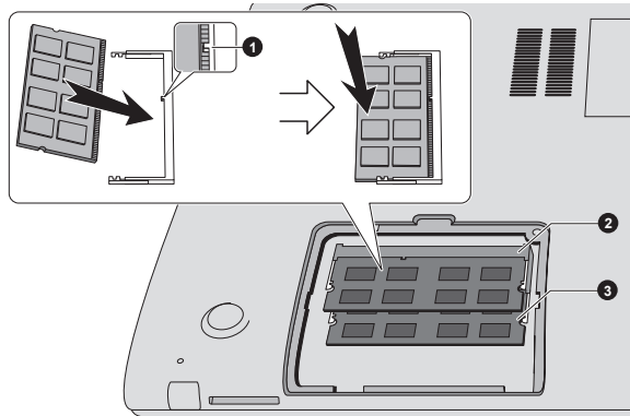
Figure 4-7 Seating the memory module
