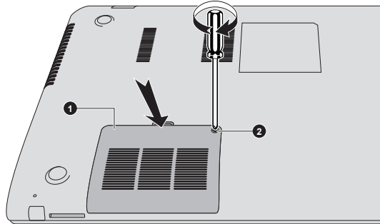
Figure 4-8 Seating the memory module cover
