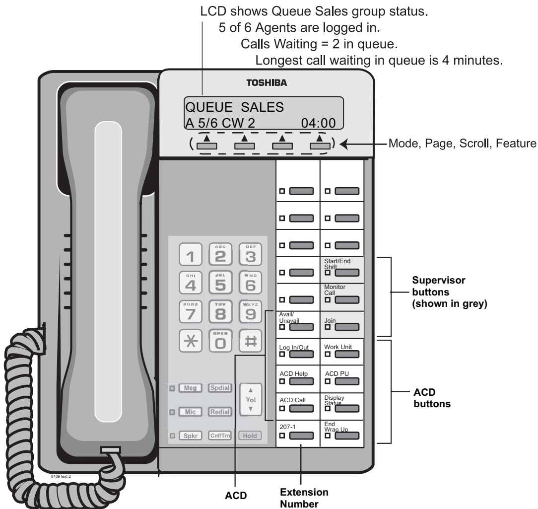
Figure 1 DKT3200-series LCD Telephone with ACD Buttons
