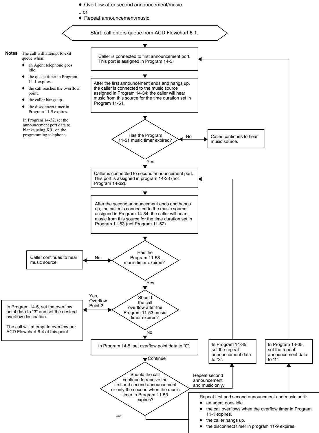
Flowchart 6-9 ACD Queue Pattern Configuration – Two Announcements
