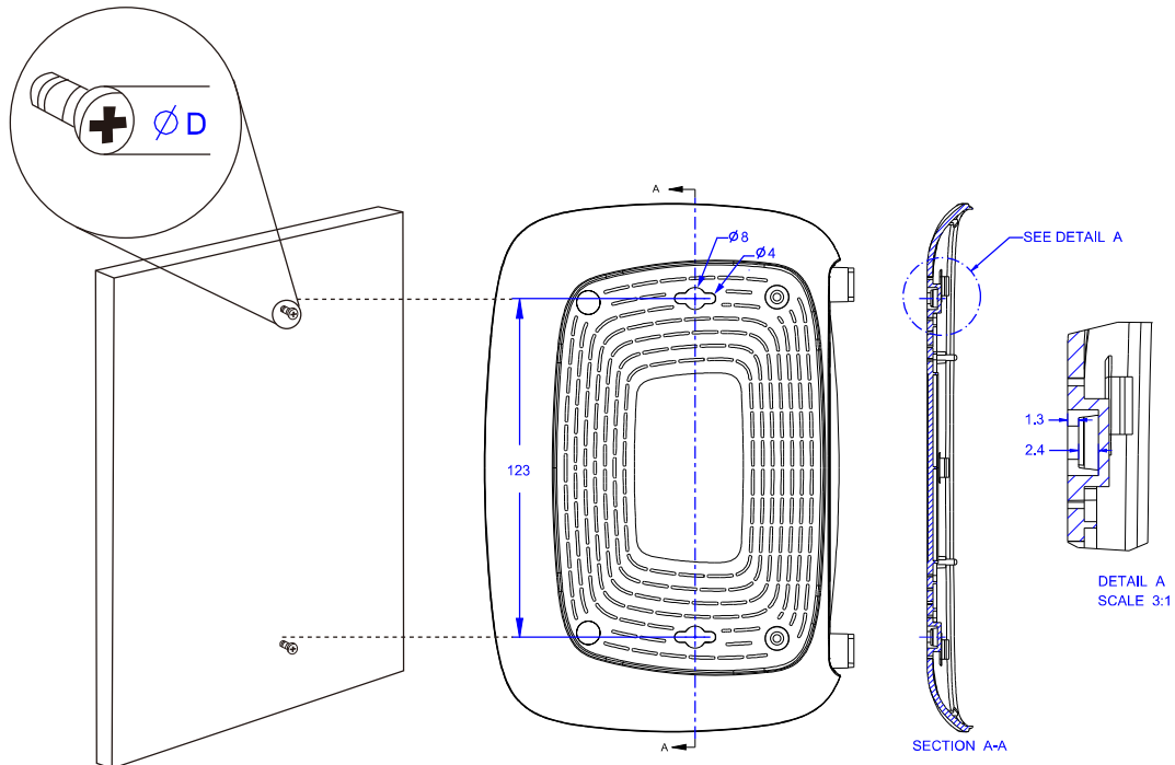
Figure 2-2 Wall-mount Install
