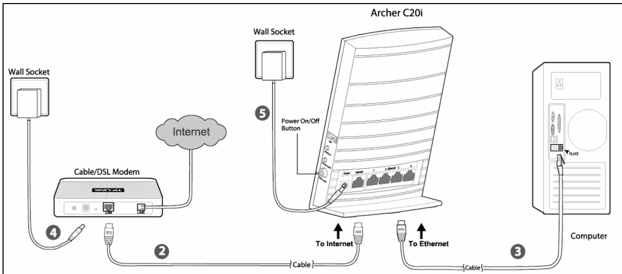
Figure 2-1 Hardware Installation
