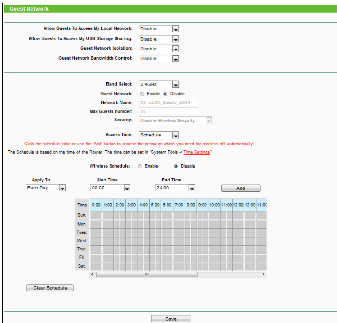
Figure 4-43 Guest Network Wireless Settings
