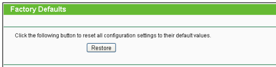
Figure 4-118 Factory Defaults
