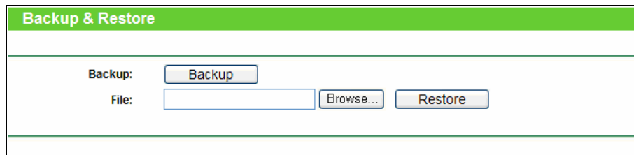
Figure 4-119 Backup & Restore
