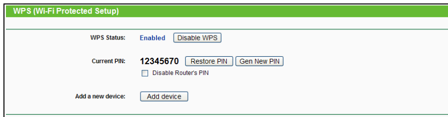
Figure 4-29 WPS
