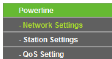
Figure 4-41 Powerline menu
