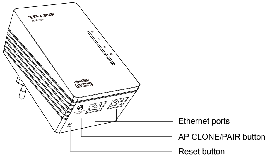
Figure 1-5 Bottom panel
