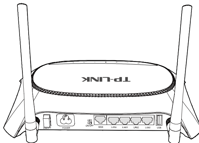
Figure 1-2 Rear panel
