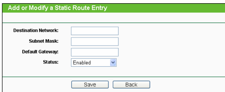
Figure 4-98 Add or Modify a Static Route Entry
