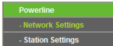
Figure 5-6 Powerline menu
