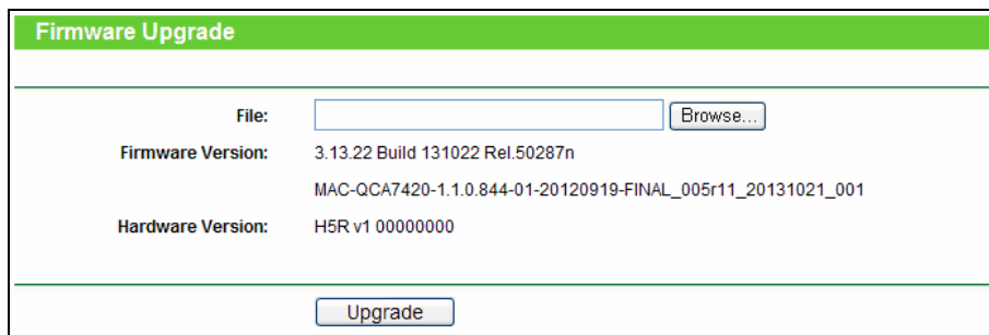
Figure 4-117 Firmware Upgrade
