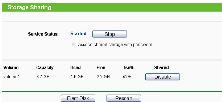
Figure 4-54 Storage Sharing
