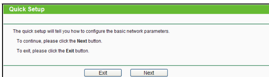
Figure 3-5 Quick Setup
