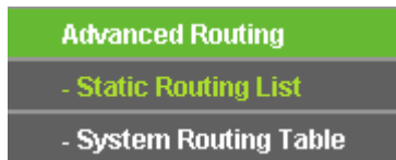
Figure 4-96 Advanced Routing
