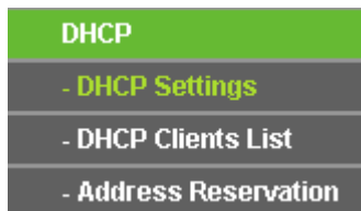
Figure 4-48 DHCP menu
