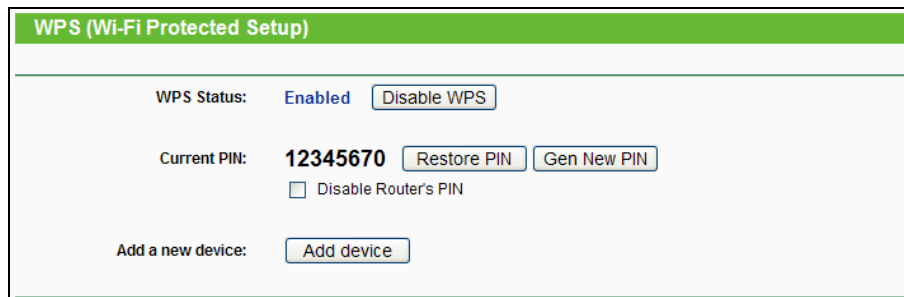
Figure 4-15 WPS
