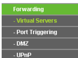
Figure 4-66 Forwarding menu
