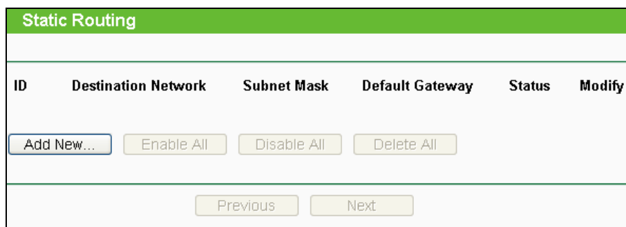
Figure 4-97 Static Routing
