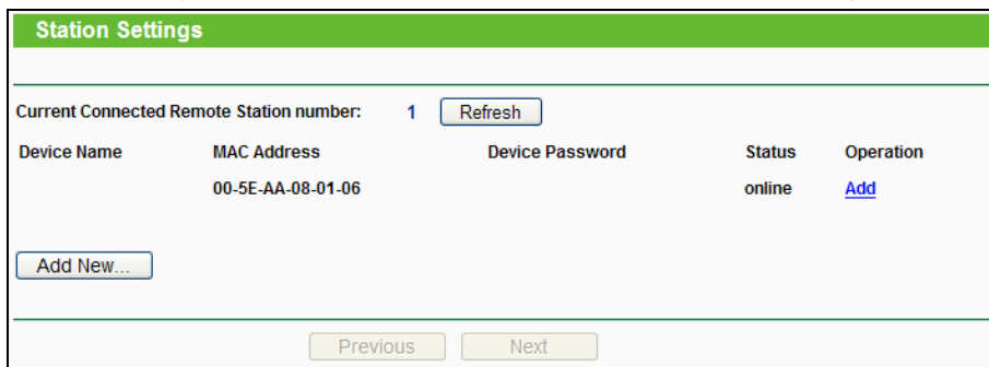
Figure 4-43 Station Settings
