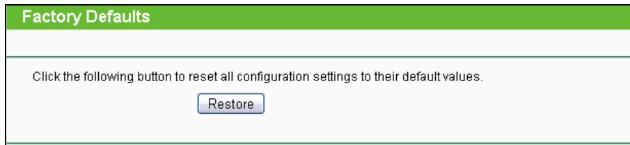
Figure 5-13 Factory Defaults
