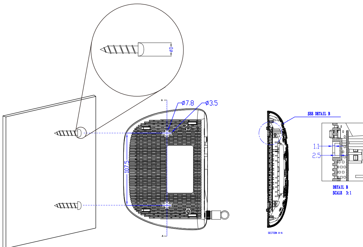
Figure 2-1 Wall-mount Install
