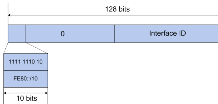
Figure 4-9 Link-local Address Format
