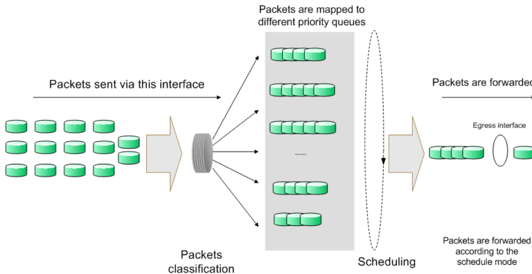
Figure 9-1 QoS function
