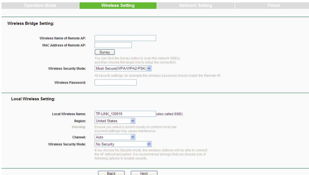
Figure 3-8 Wireless Setting – Bridge with AP mode
