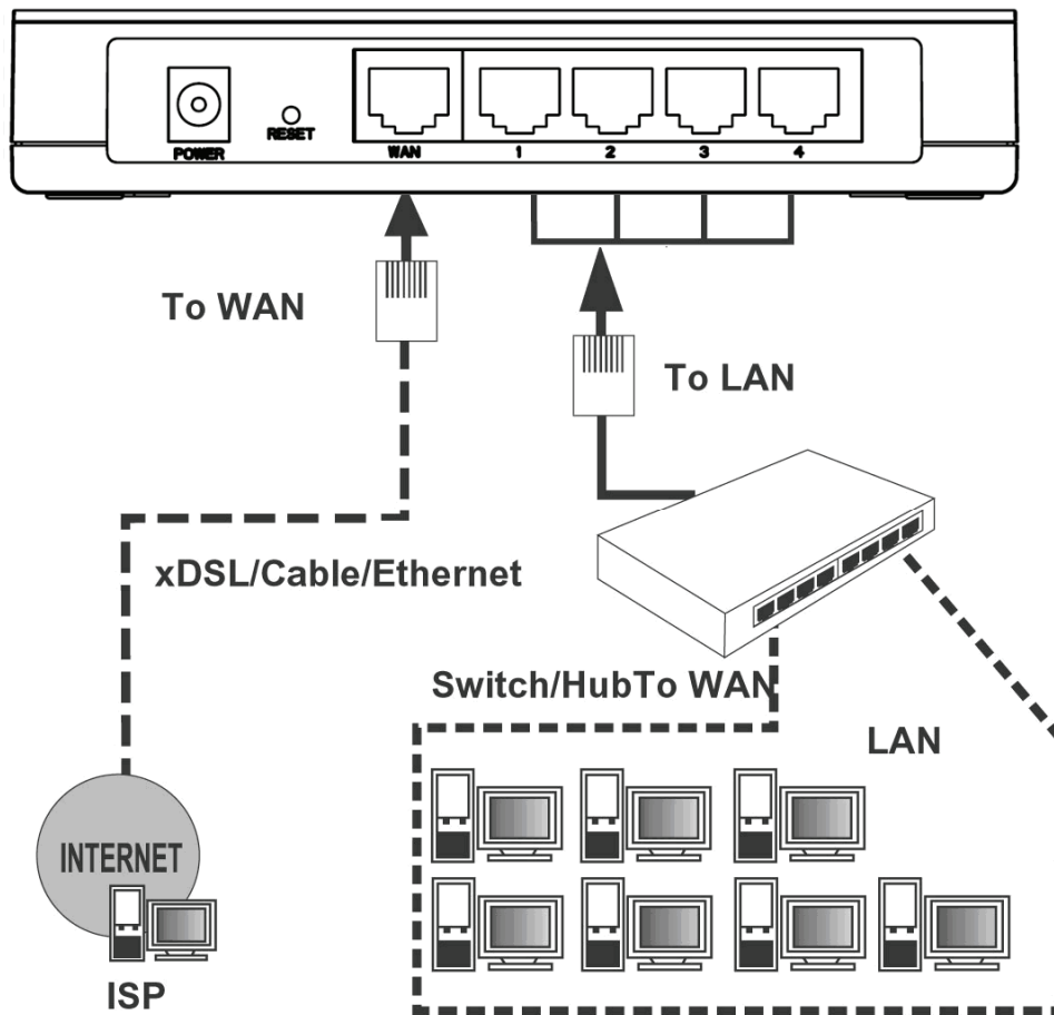
Figure 2-1 Hardware Installation of the TL-R402M Cable/DSL Router
