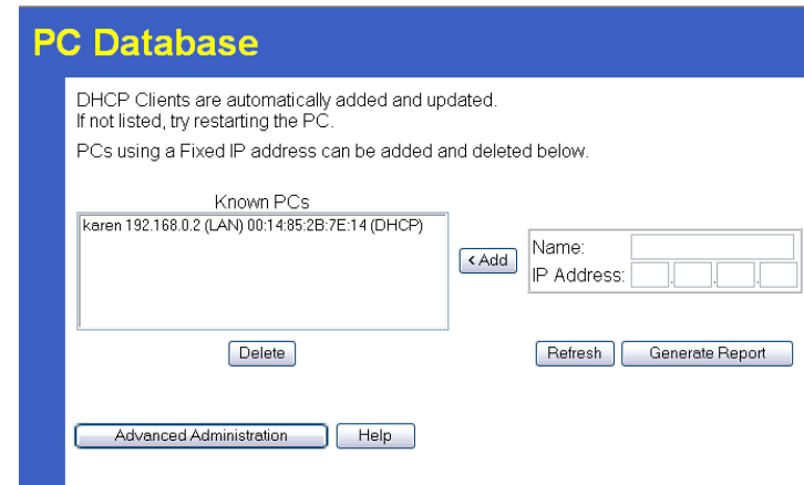
Figure 44: PC Database
