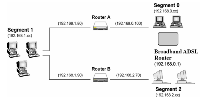
Figure 52: Routing Example
