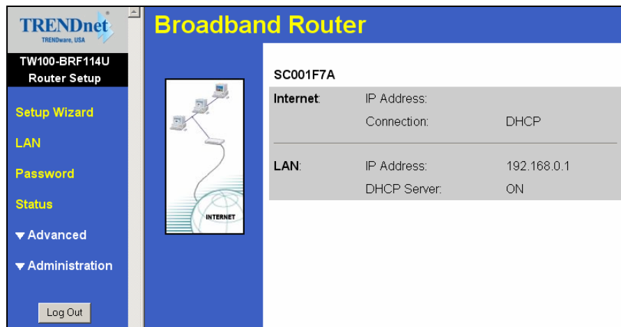
Figure 5: Home Screen
