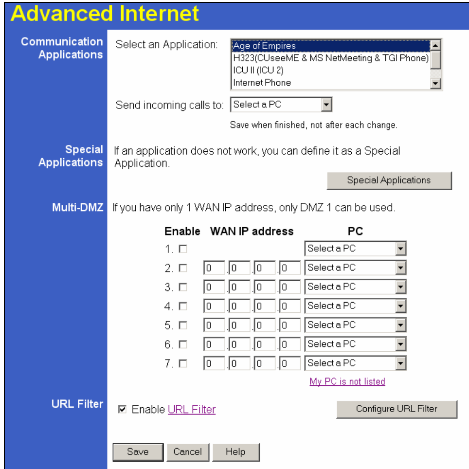
Figure 38: Internet Screen
