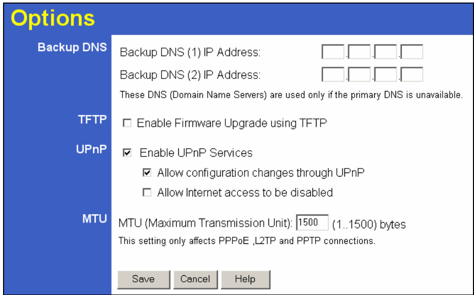
Figure 47: Options Screen
