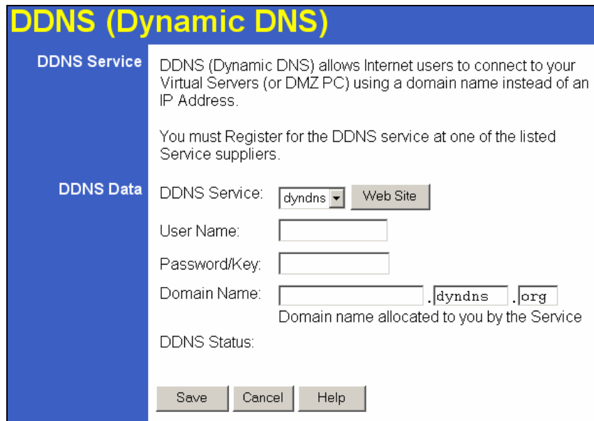
Figure 37: DDNS Screen
