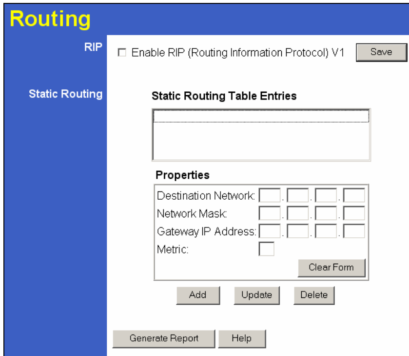
Figure 51: Routing Screen
