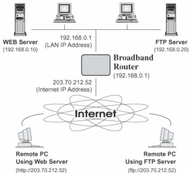
Figure 41: Virtual Servers
