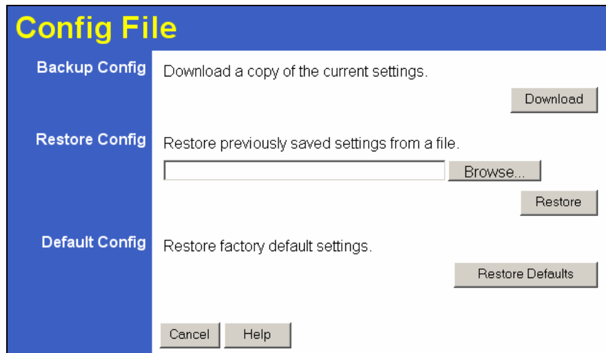
Figure 44: Config Screen
