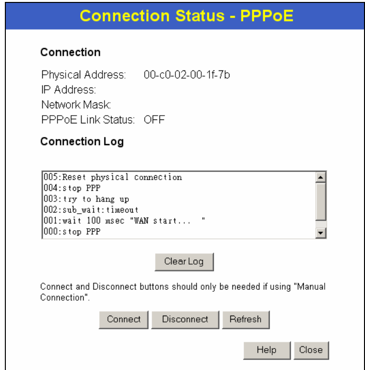
Figure 28: PPPoE Status Screen
