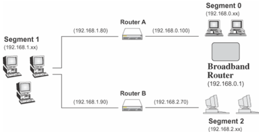
Figure 52: Routing Example
