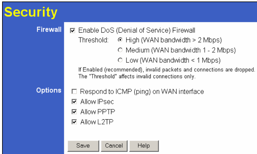
Figure 53: Security Screen
