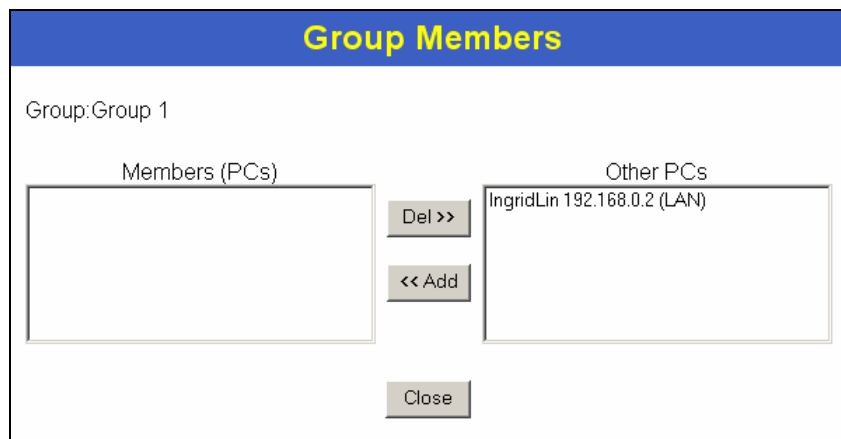
Figure 34: Group Members
