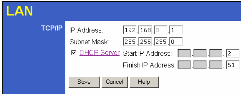
Figure 6: LAN Screen
