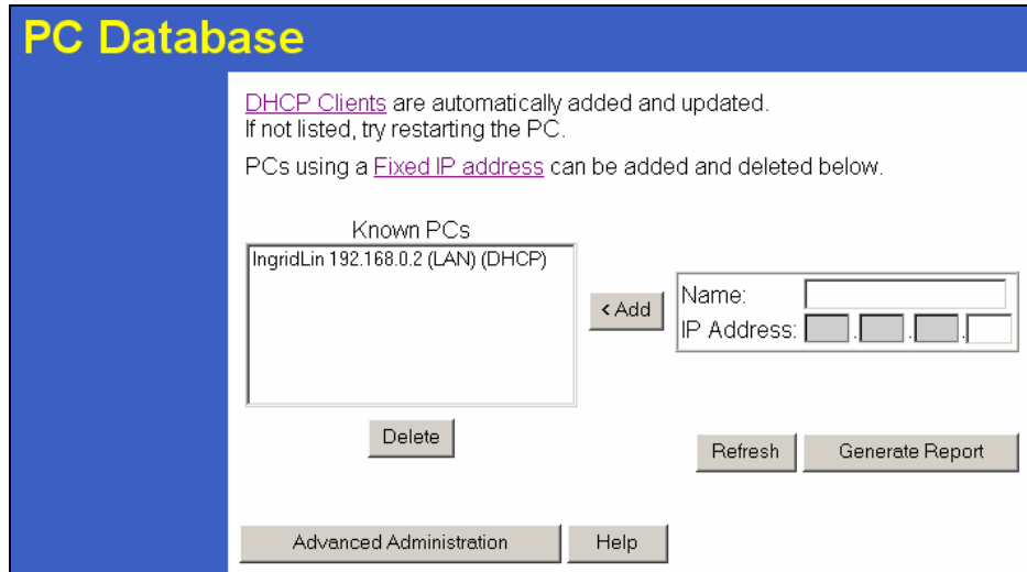
Figure 48: PC Database
