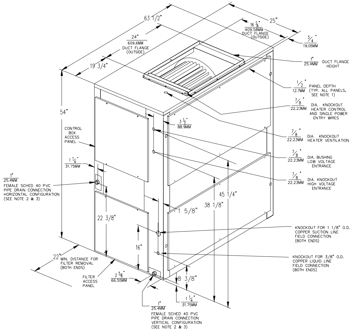
Figure DD-7—TWE100A Air Handler All dimensions are in inches and millimeters.
