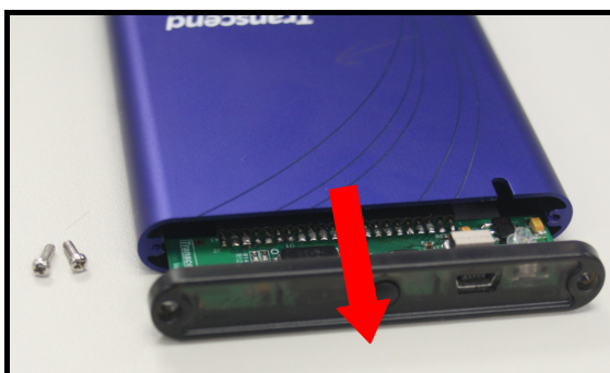
Figure 3. Remove the top cover revealing the IDE adapter
