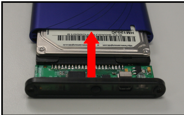
Figure 5. Reinsert the adapter plus drive and reattach the screws
