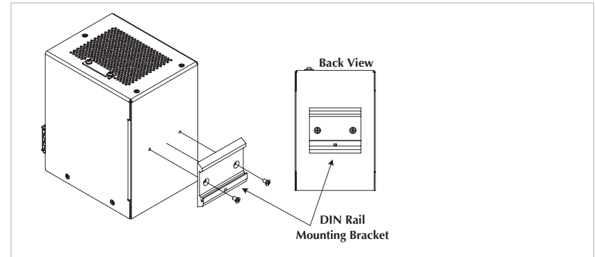
Figure 8: DIN-Rail Bracket
