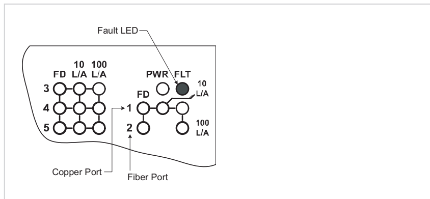
Figure 13: Fault LED
