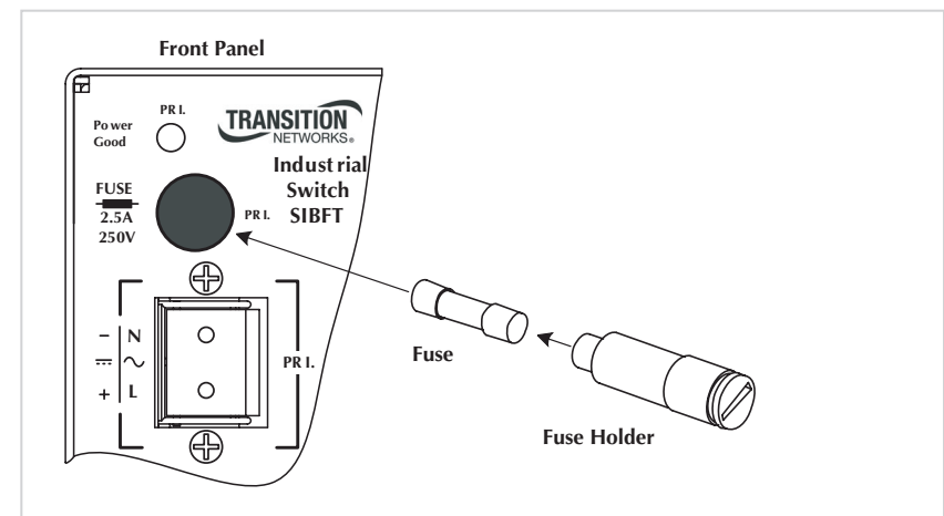
Figure 15: Fuse Replacement
