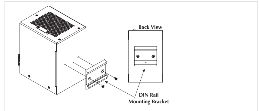
Figure 8: DIN-Rail Bracket
