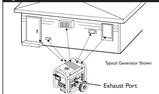
Figure 3 — Generator Clearance
