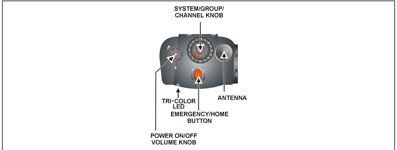
Figure 8-1: Top View
