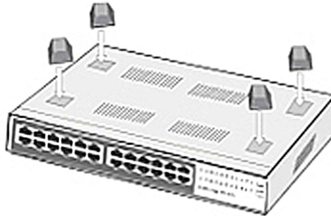
Figure 2-4. Attaching Rubber Feet to each corner on the bottom of the Switch
