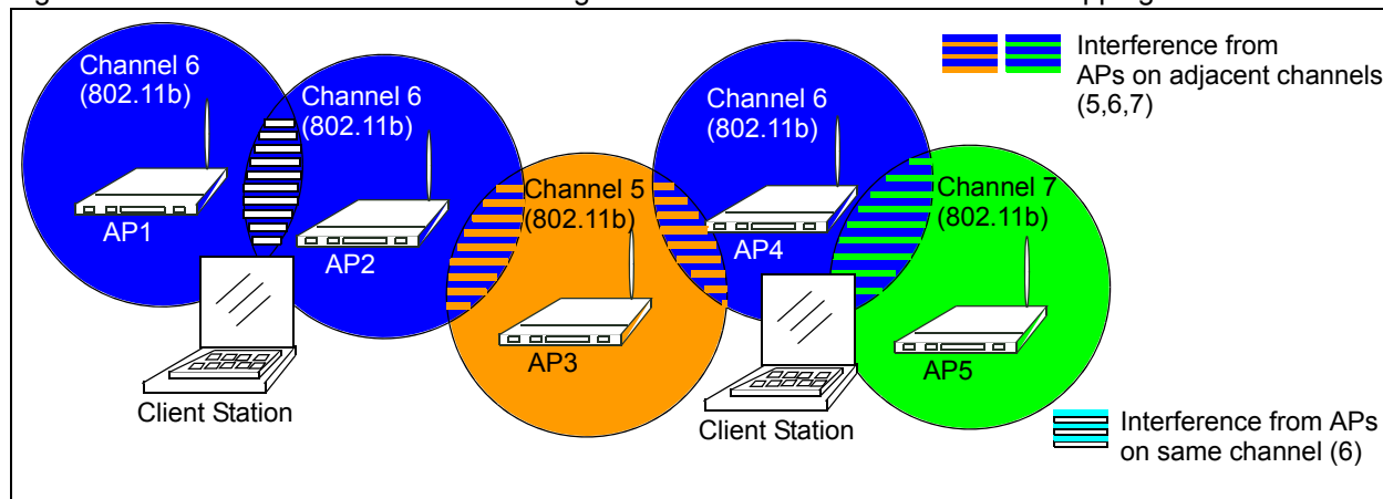
Figure 3. Without Automatic Channel Management: APs Can Broadcast on Overlapping Channels.
