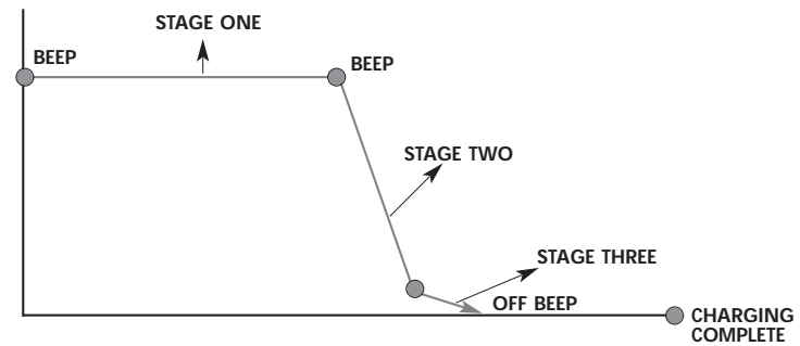
Charge Curve
