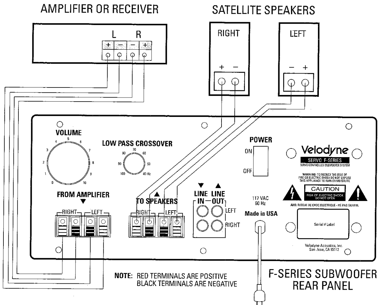
Figure 1: Installation Using FROM AMPLIFIER Inputs
