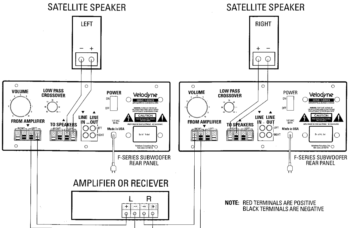
Figure 3: Installation Using STEREO SUBWOOFERS
