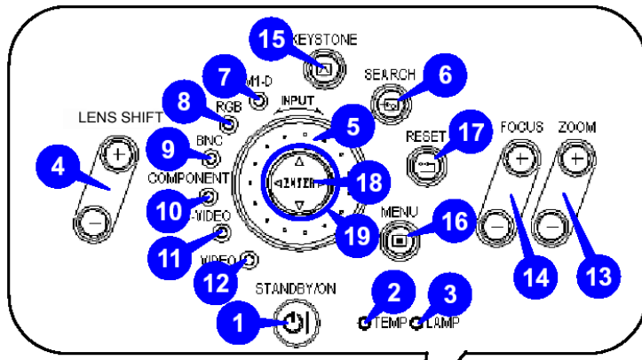
Control Panel on the Projector
