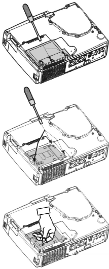
Figure 7: Lamp Replacement
