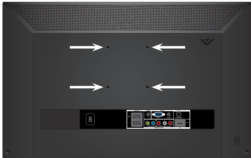
WALL MOUNT SCREW LOCATIONS
