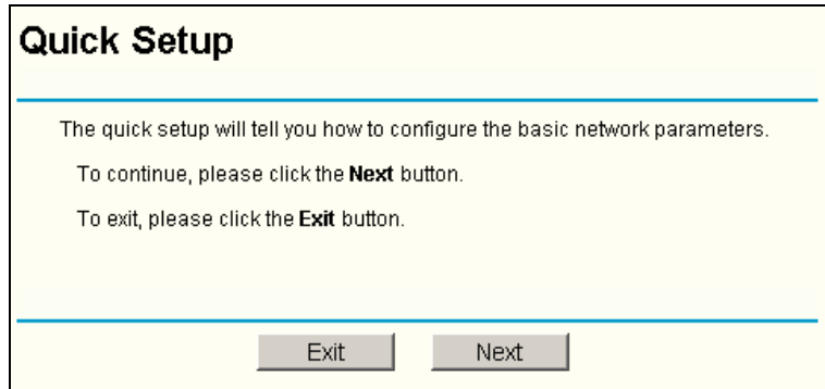
Figure 4-5 Quick Setup
