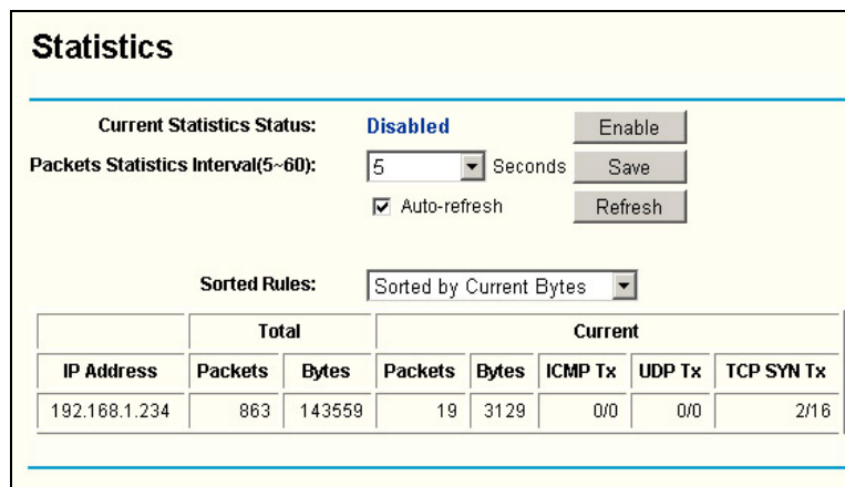
Figure 5-42 Statistics
