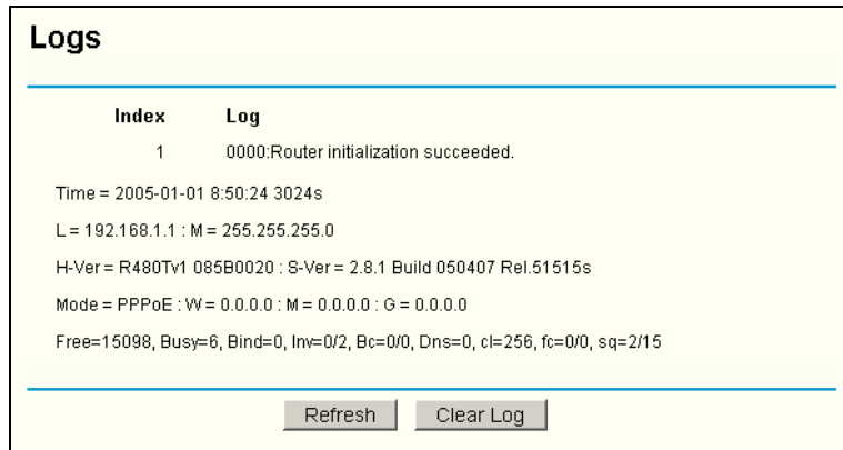
Figure 5-41 System Log
