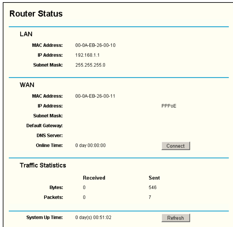
Figure 5-1 Router Status
