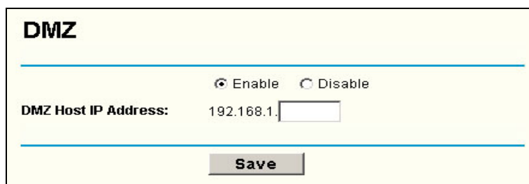
Figure 5-19 DMZ
