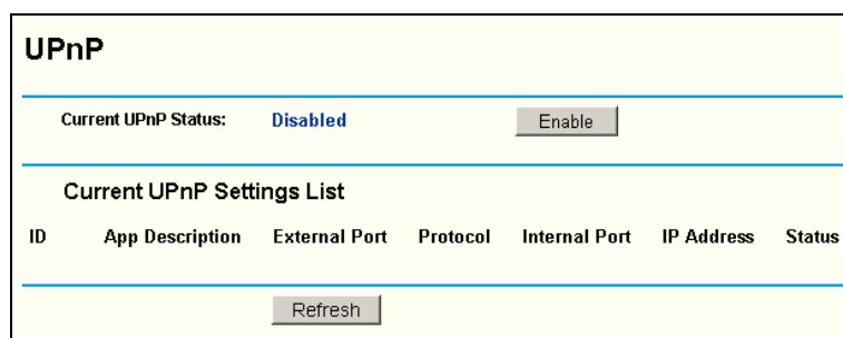
Figure 5-20 UPnP Settings
