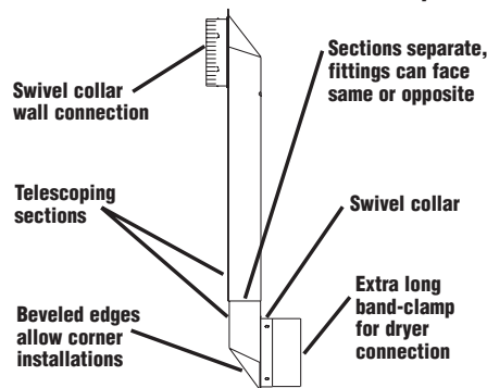
Part #4396037
