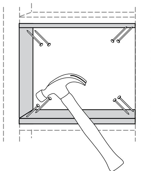
Frame the hole with two-by-four supports
