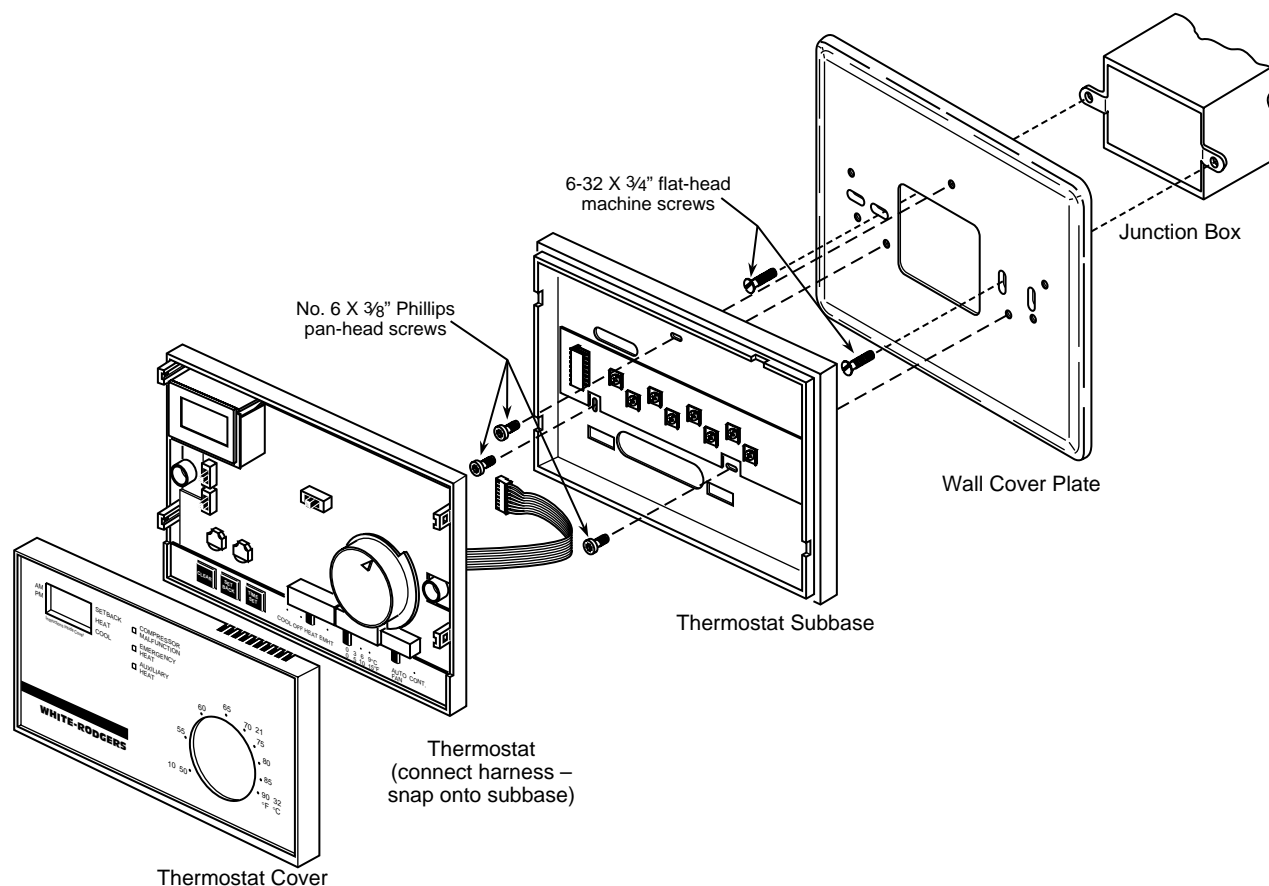
Figure 10. Mounting 1F62 thermostat to horizontal junction box
