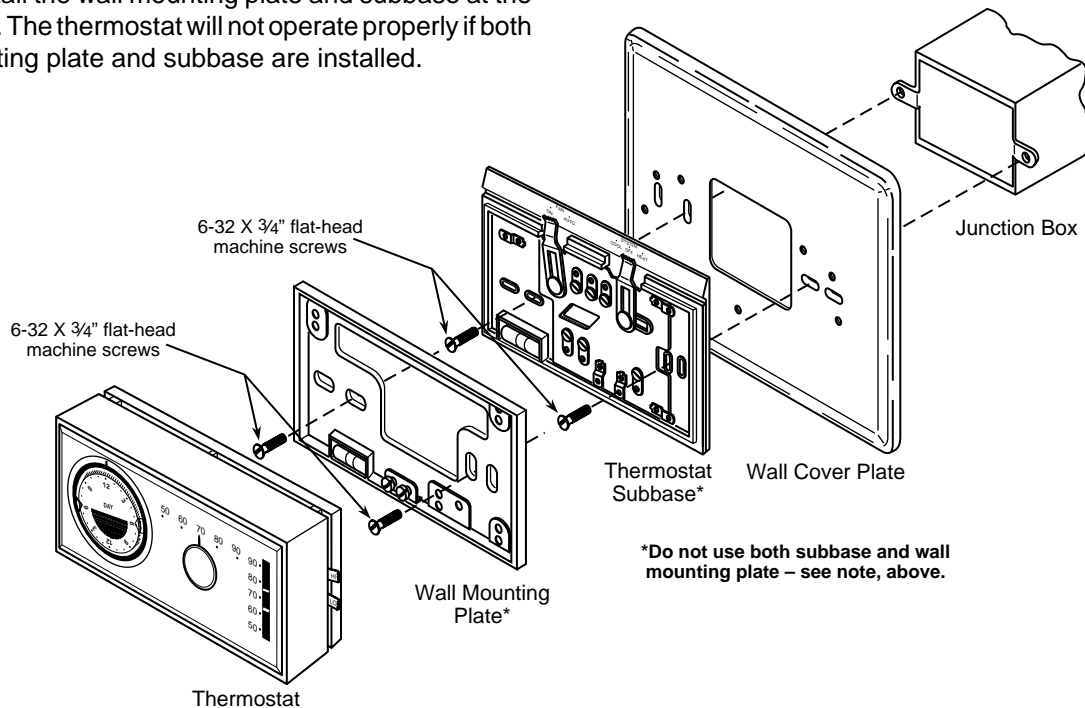
Figure 4. Mounting 1F7X quartz clock thermostat to horizontal junction box
