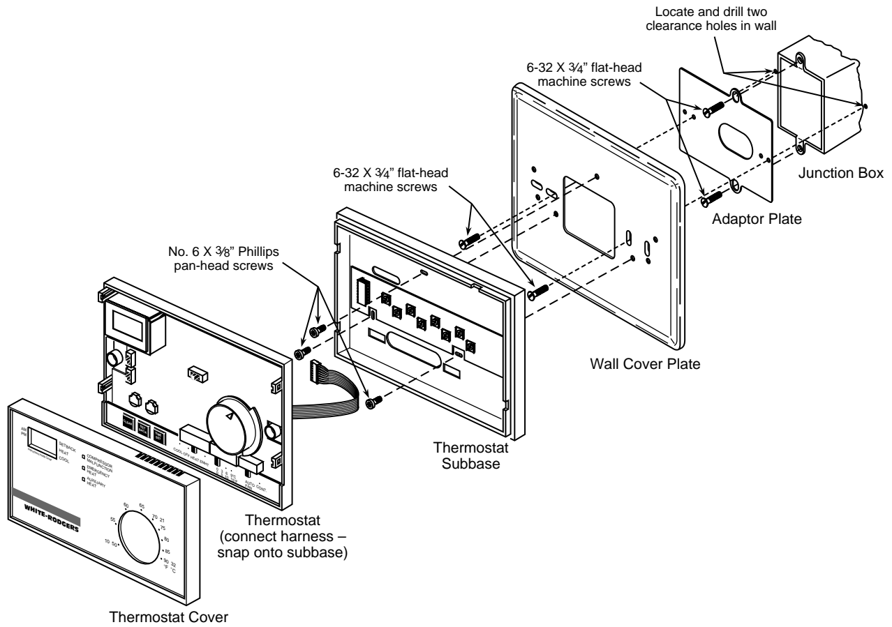
Figure 11. Mounting 1F62 thermostat to vertical junction box
