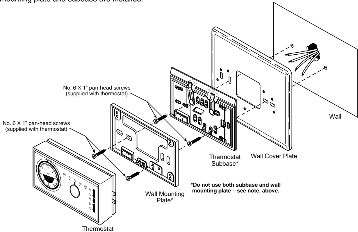
Figure 6. Mounting 1F7X quartz clock thermostat to wall
