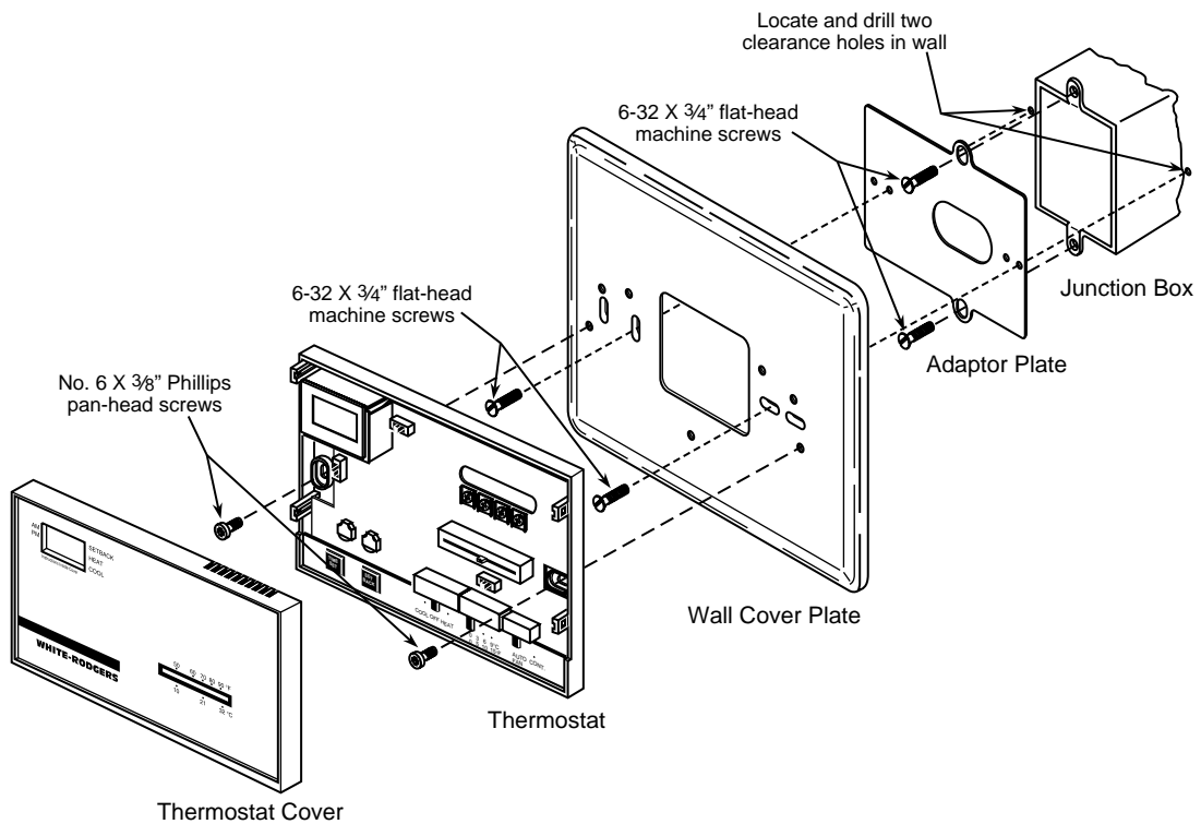
Figure 8. Mounting 1F60 thermostat to vertical junction box
