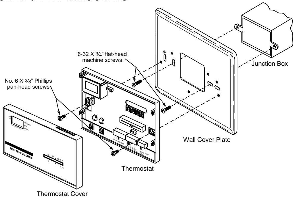
Figure 7. Mounting 1F60 thermostat to horizontal junction box
