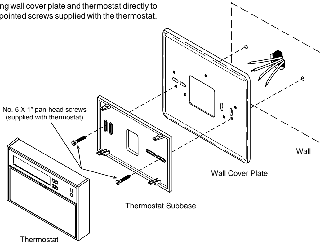
Figure 3. Mounting 1F9X digital thermostat to wall
