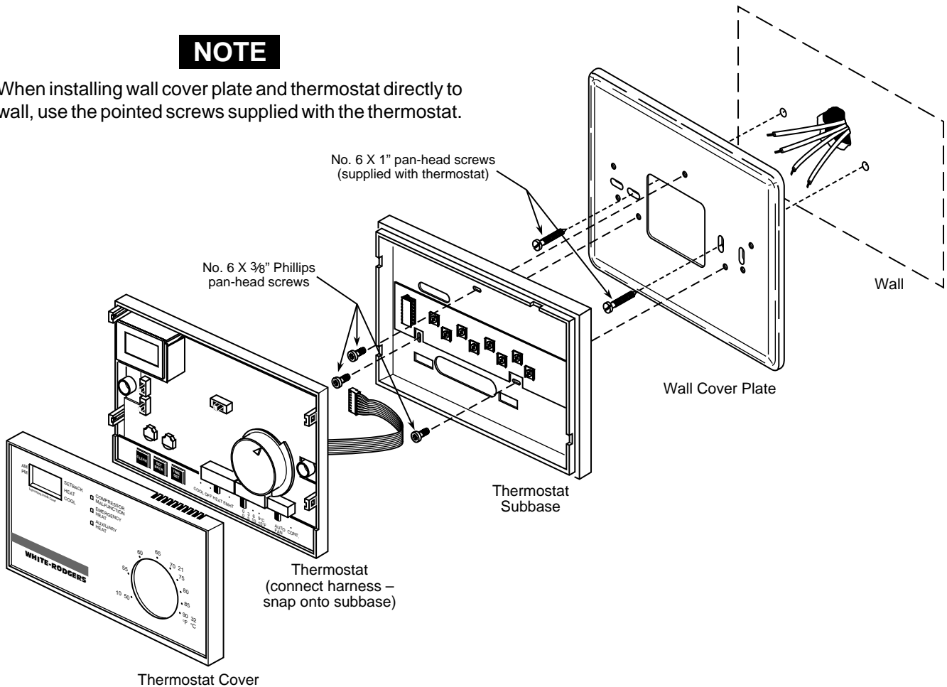
Figure 12. Mounting 1F62 thermostat to wall
