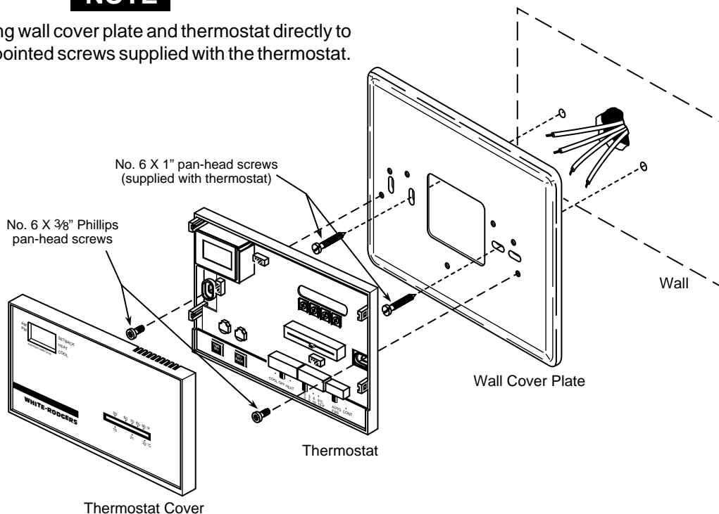
Figure 9. Mounting 1F60 thermostat to wall
