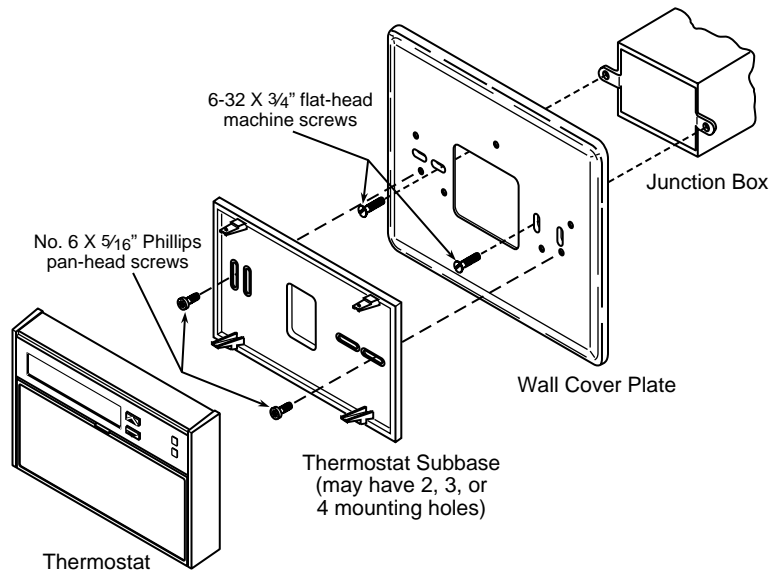
Figure 1. Mounting 1F9X digital thermostat to horizontal junction box
