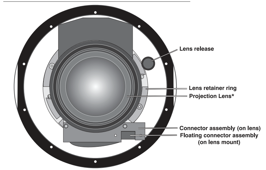
Figure 4.8. Lens Assembly
