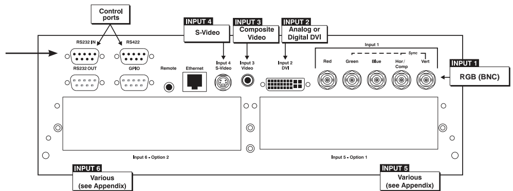
Figure 2.6 Input Panel
