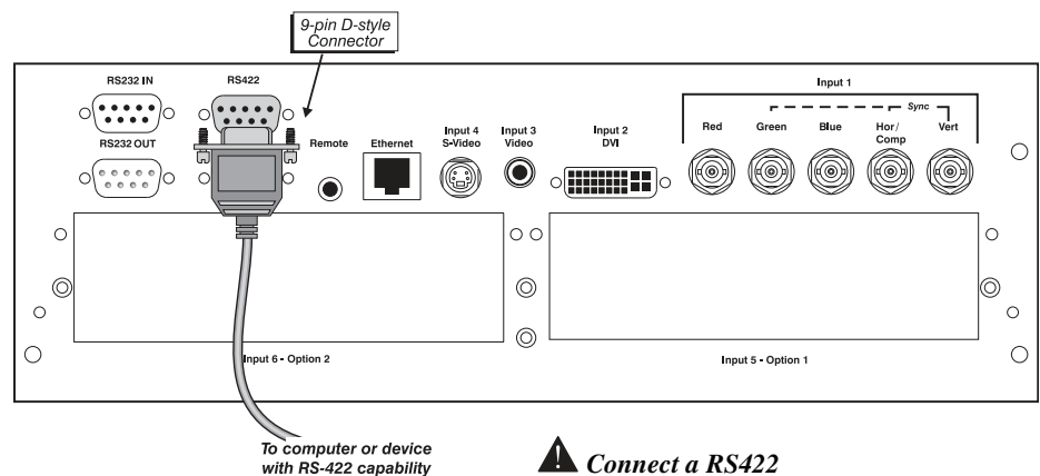
Figure 2.11 Connecting RS-422
