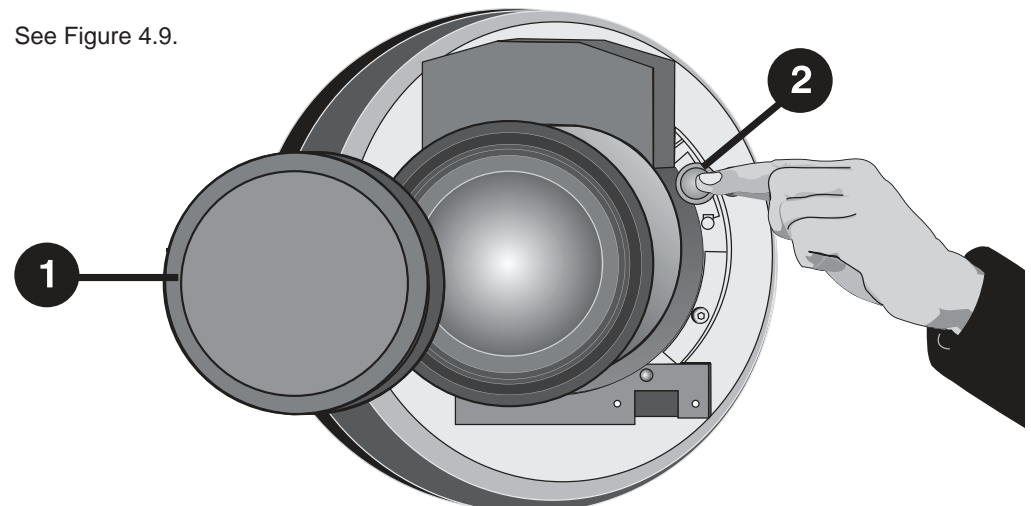
Figure 4.9. Depressing Lens Release
