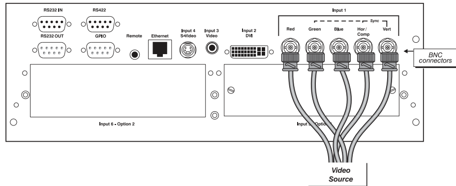
Figure 2.7 Connecting RGB and Sync
