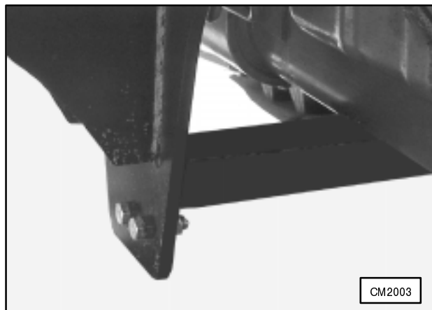
Figure 4. Install Crossmember
