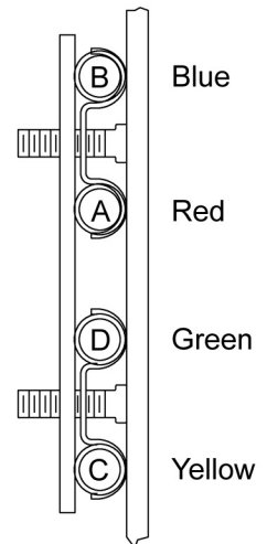
Figure 12. Loader Feedline Identification
