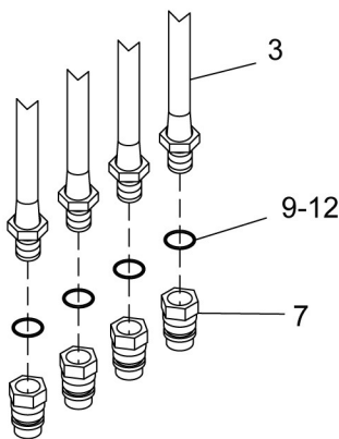
Loader Feedline Hoses
