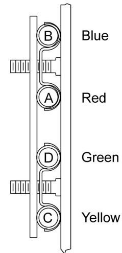
LUP126-2 or LUP132-2 Loader Feedlines
