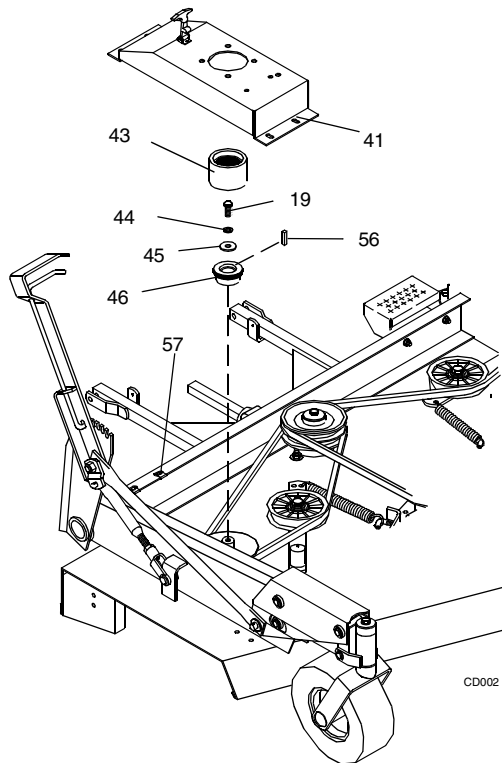
Figure 6. Bearing Mount Assembly Installation
