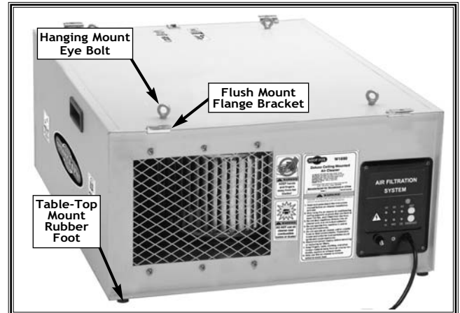
Figure 4. Air cleaner unit mounting options.
