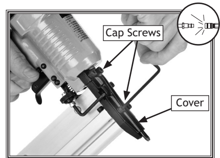
Figure 7. Opening cover to clear a jam.
