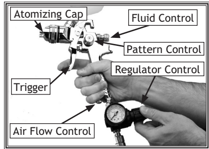
Figure 4. Controls.
