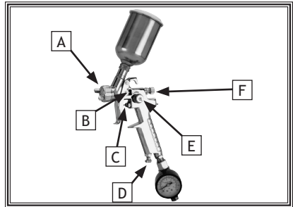
Figure 11. Lubrication points.
