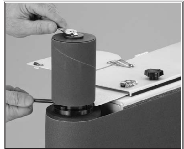
Figure 18. Anchoring the spindle with the rod.
