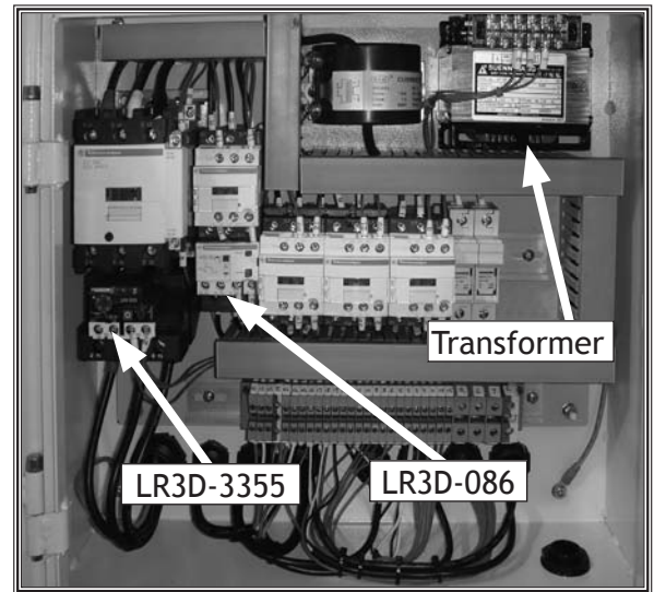
Figure 6. Overload relay and transformer location.
