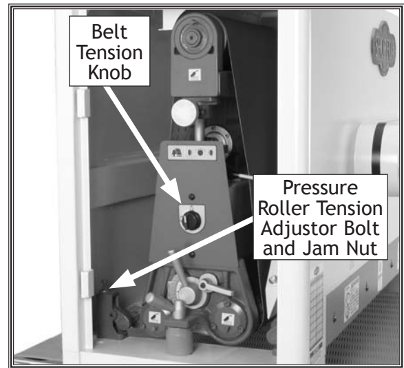
Figure 51. Belt and pressure roller adjustments.
