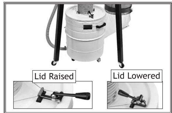
Figure 24. Drum positioning at front of machine.
