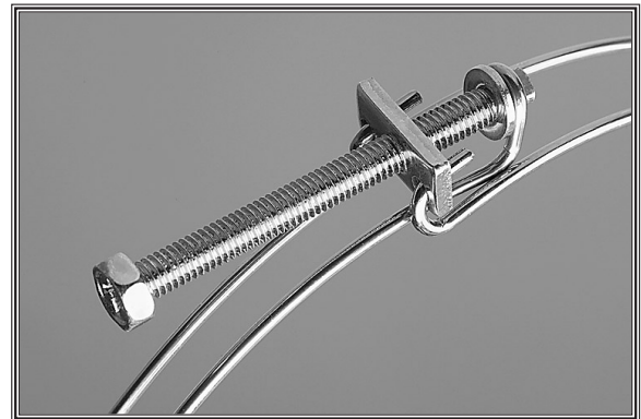
Figure 19. Correct hose clamp assembly.
