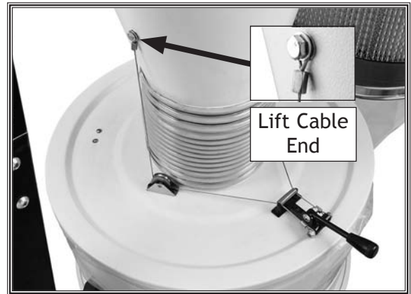
Figure 18. Collection lid installation.
