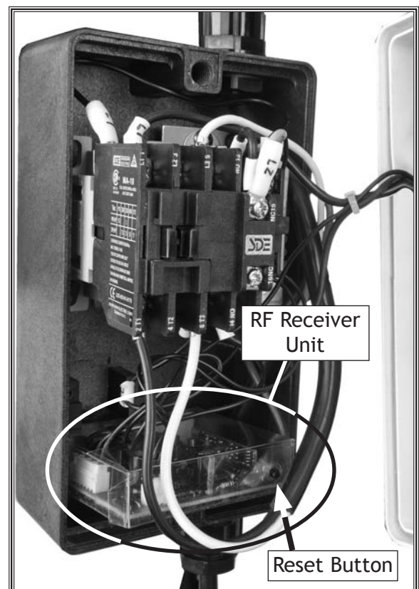
Figure 38. Remote control receiver.
