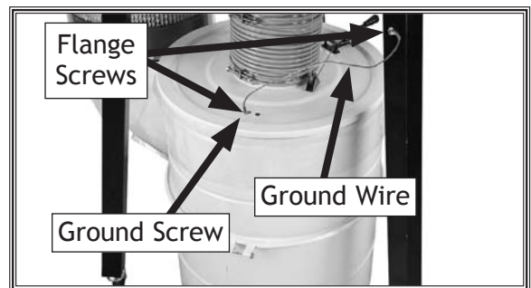
Figure 20. Ground wire location.
