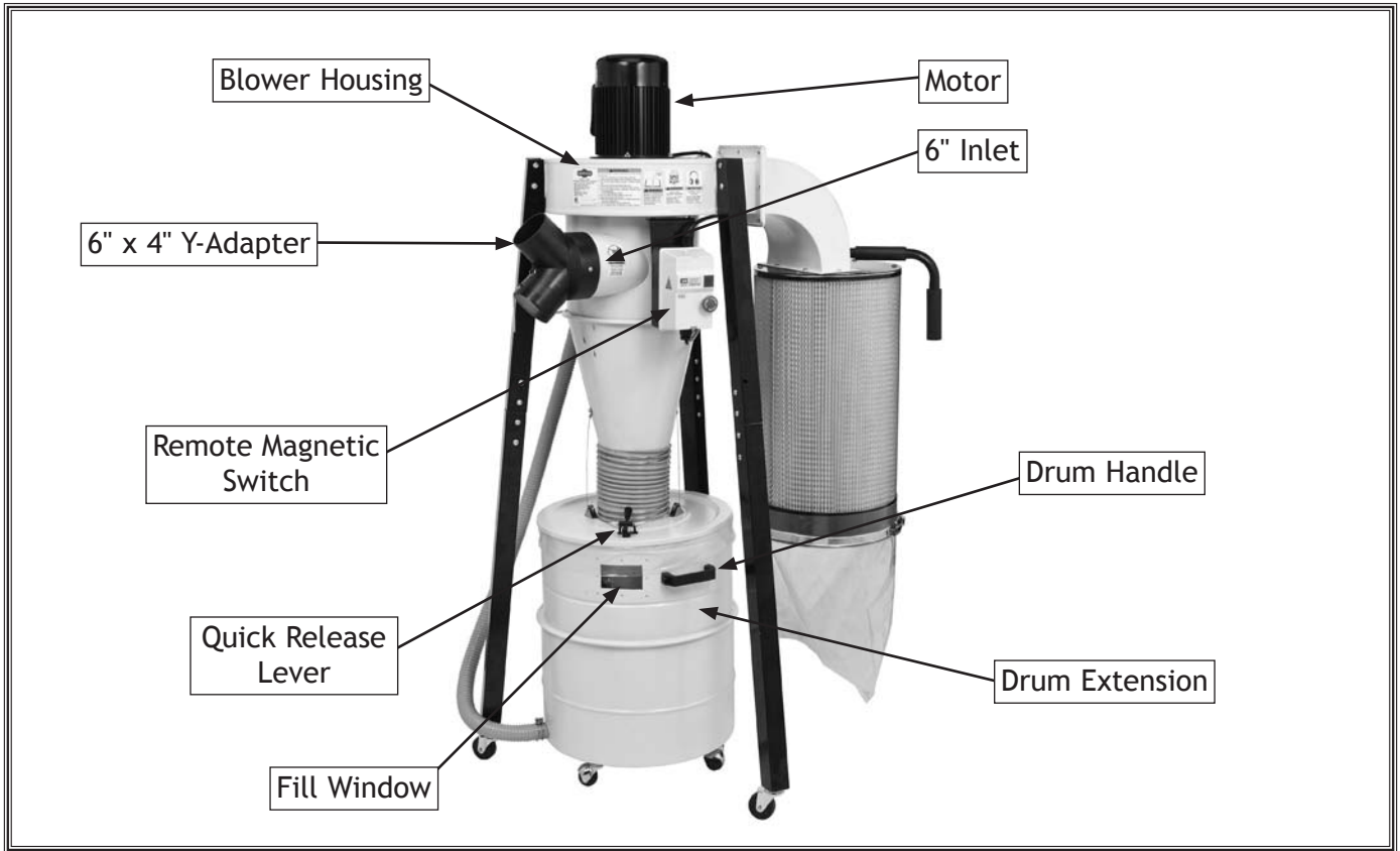
Figure 1. Right side view.
