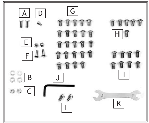
Figure 6. Hardware and tool bag inventory.
