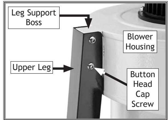
Figure 9. Upper leg installed on blower housing leg support boss.
