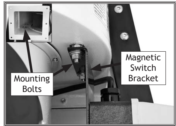
Figure 12. Magnetic switch installation.
