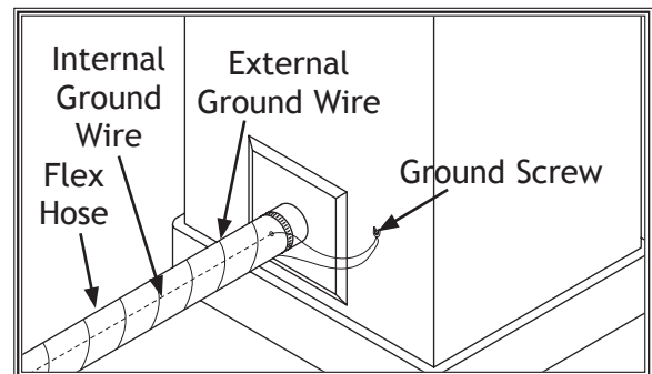
Figure 29. Flex-hose grounded to machine.
