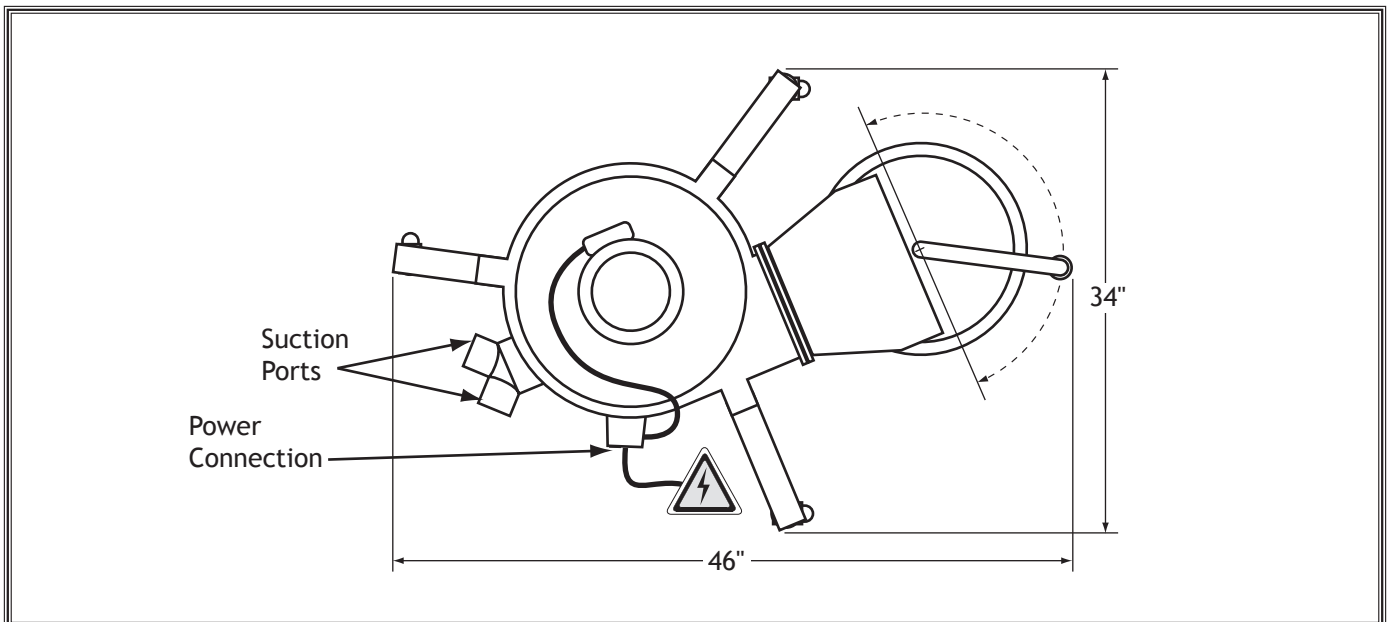
Figure 8. Model W1823 working clearances.
