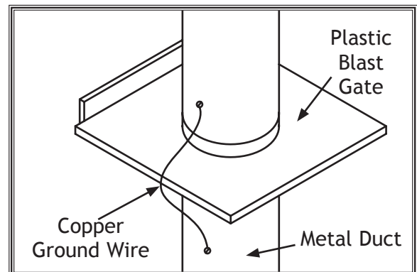
Figure 30. Ground jumper wire when using plastic blast gates and metal duct.
