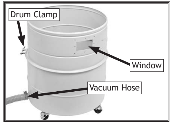
Figure 22. Drum and drum extension positioning and installation.
