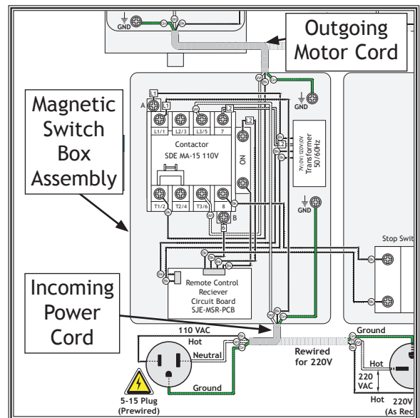
Figure 42. Magnetic switch.
