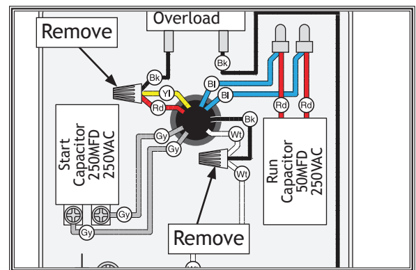
Figure 39. Motor wires at 110V.
