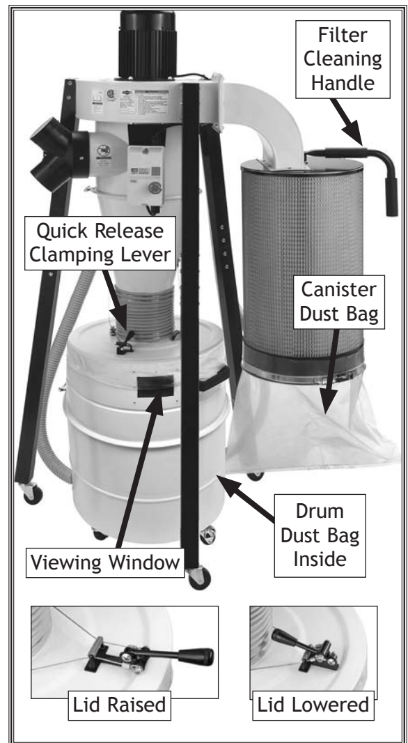
Figure 35. Maintenance locations.
