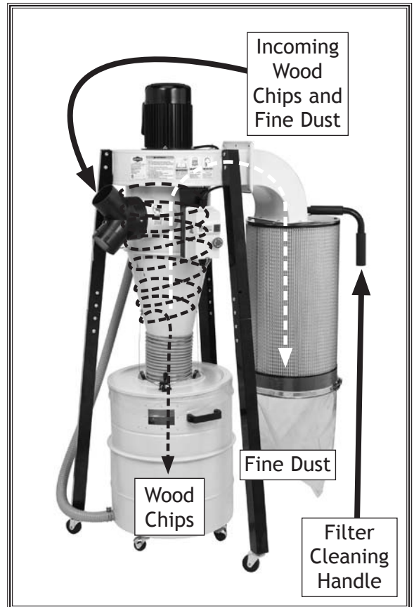
Figure 31. Model W1823 flow.
