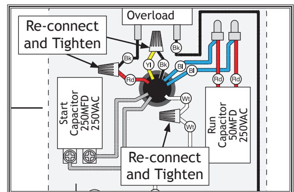
Figure 40. Motor wires re-positioned for 220V.
