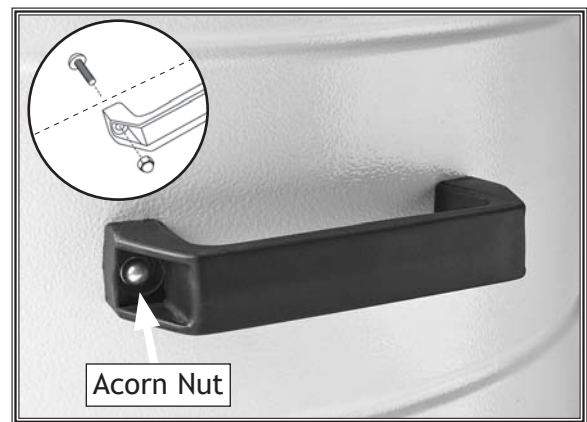
Figure 23. Handle installation.
