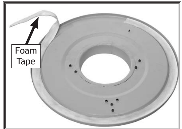
Figure 17. Collection drum cover seal and lift cable clamping location.
