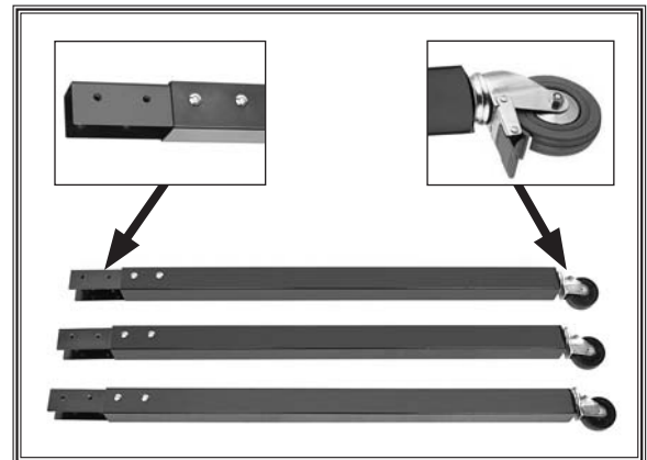
Figure 10. Lower leg connector and swivel caster installation.
