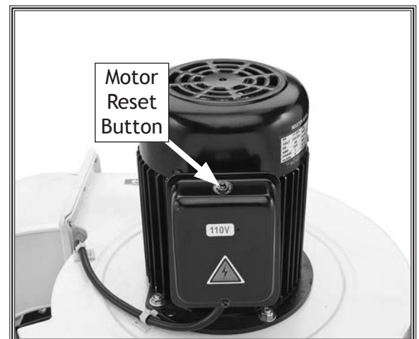
Figure 34. Reset button on motor.
