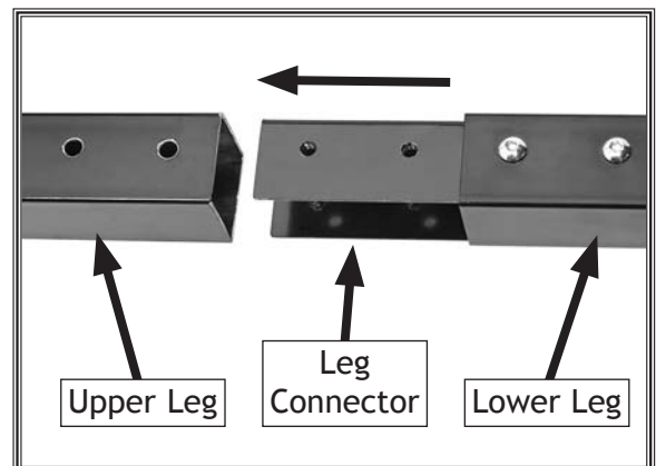
Figure 11. Inserting a lower leg into an upper leg.
