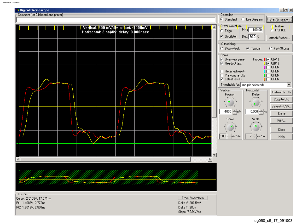
Figure 4-17: Address/Control Signals at First DDR Memory (Typical Case)
