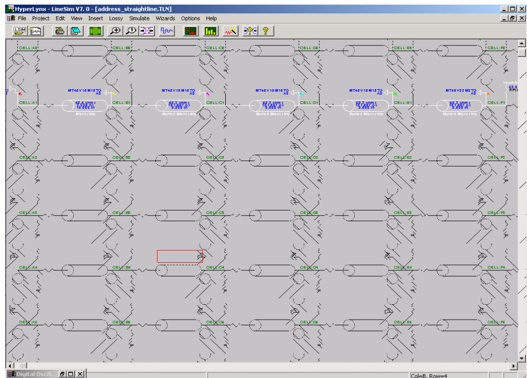
Figure 4-15: Address and Control Signal Terminations
