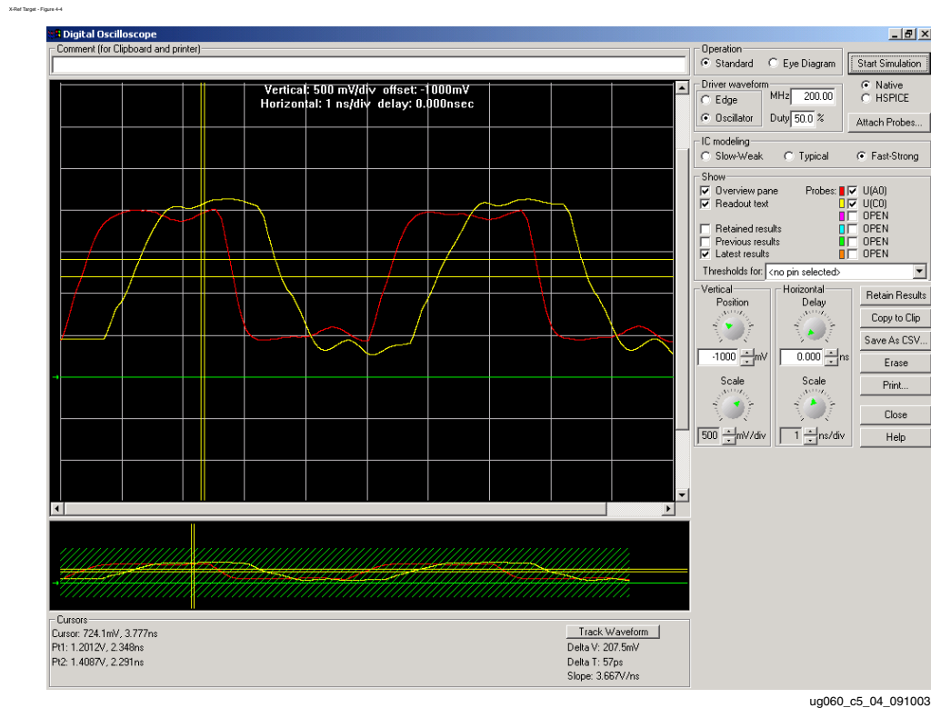
Figure 4-4: Data Signal from FPGA to Memory (Fast Strong Case)
