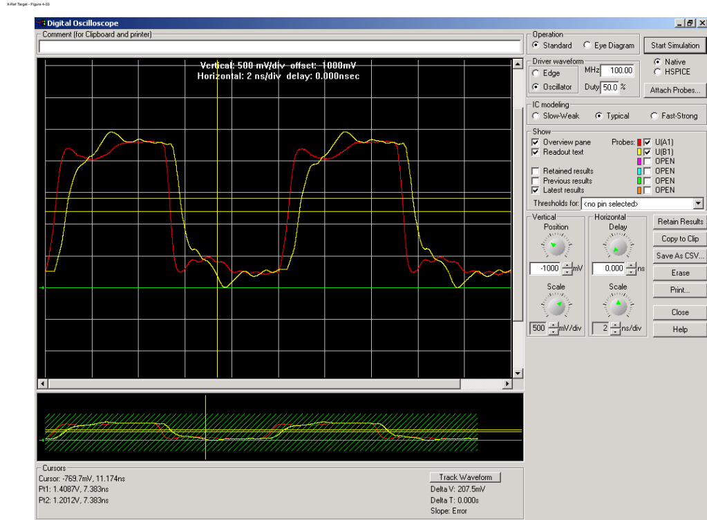
Figure 4-33: Address/Control Signals with 55Ω Impedance Measured at First DDR Component
