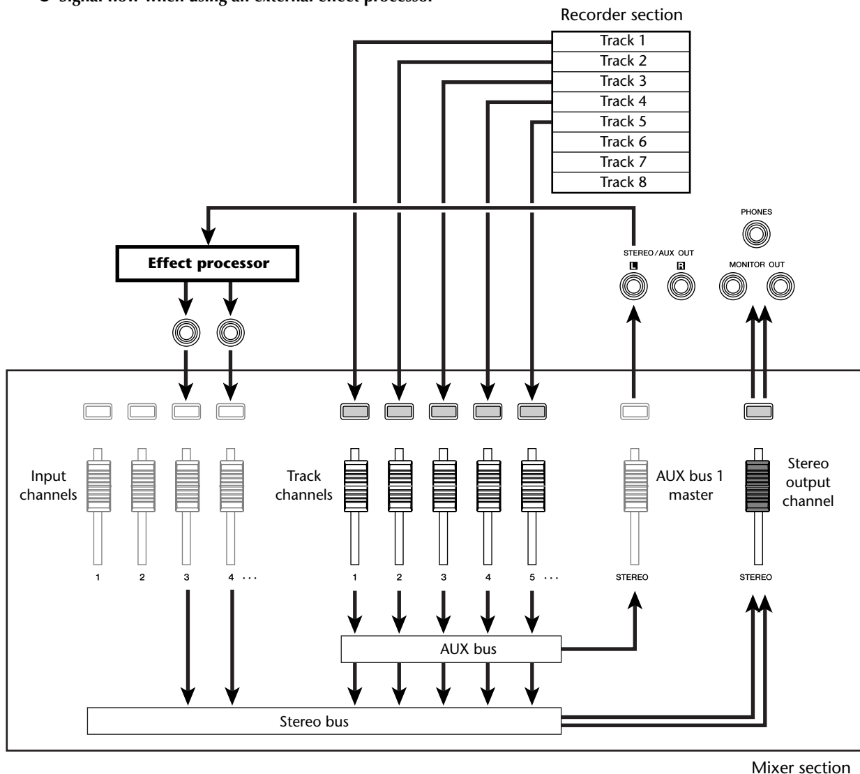
Mixer section
