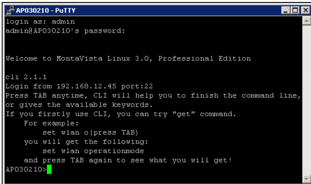
Figure 28 SSH Settings 3
