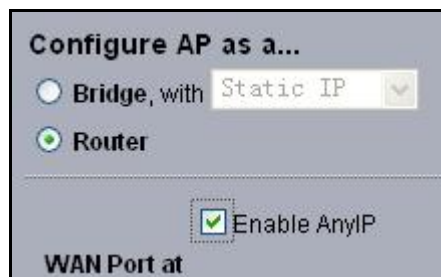
Figure 14 Any IP
