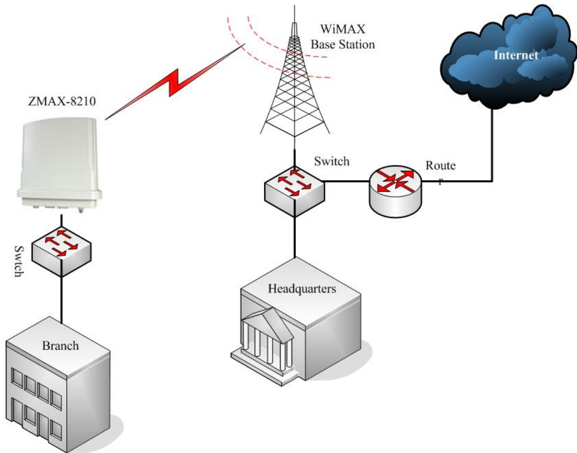
Figure 3 Wireless Point-to-Point Outdoors
