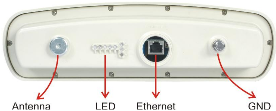
Figure 2 ZMAX-8210 ports
