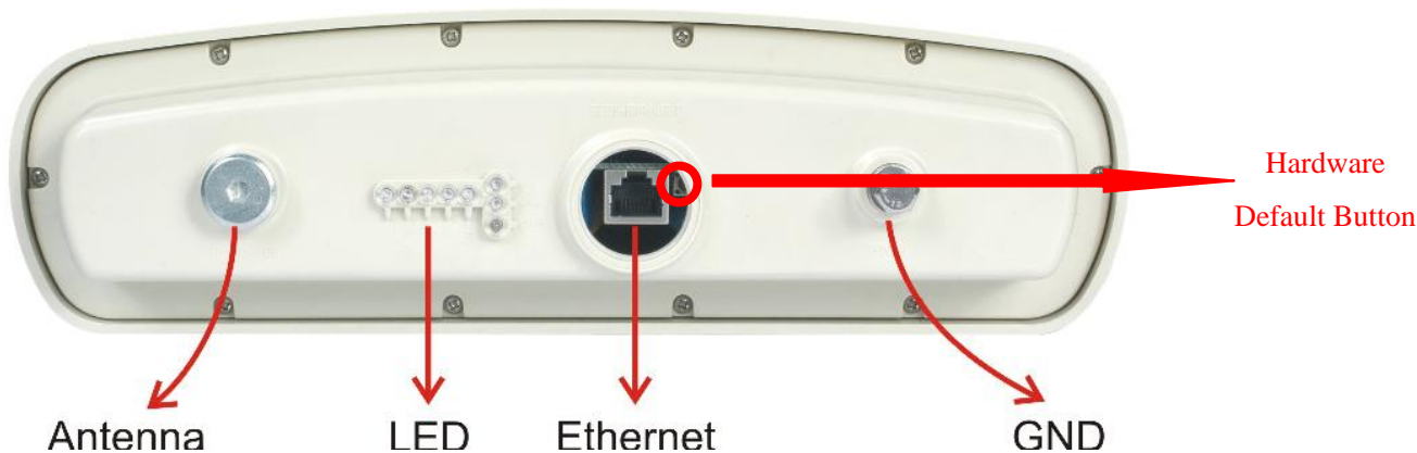
Figure 24 ZMAX-8210 Default Button
