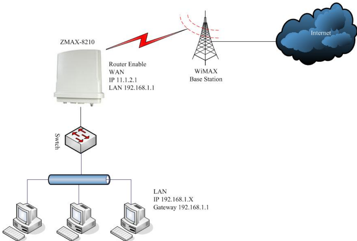
Figure 13 Wireless Router Mode
