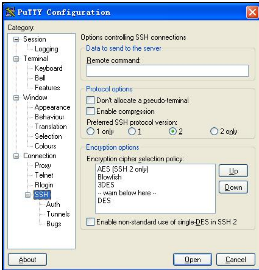
Figure 27 Putty settings 2
