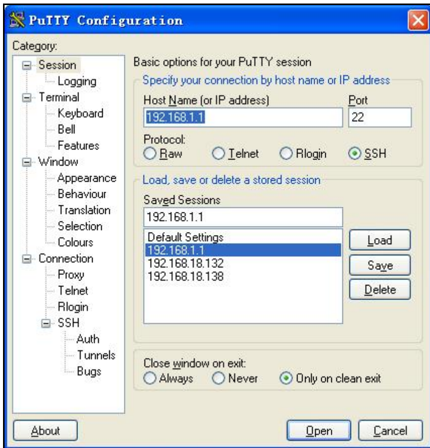
Figure 26 Putty Settings
