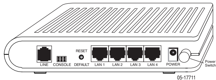
Figure 2: Back Panel
