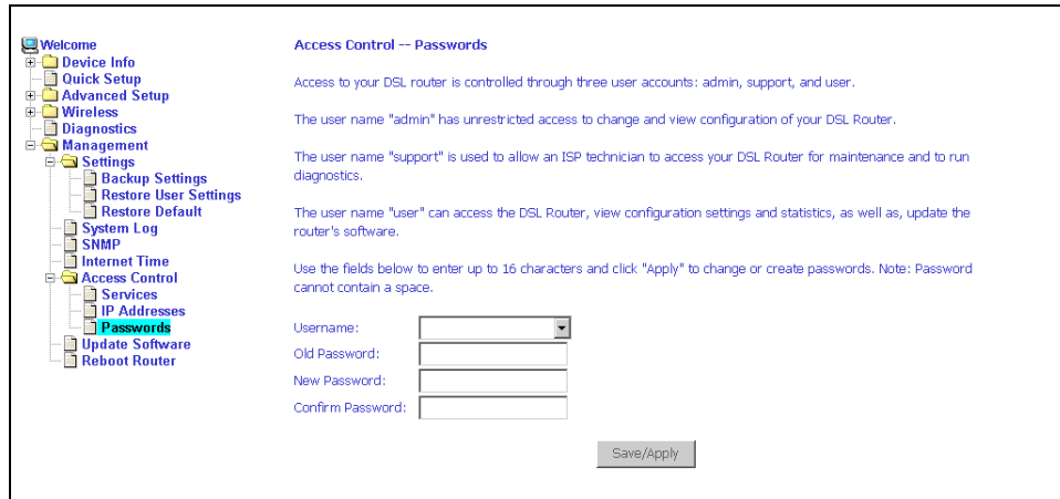
Figure 90: Access Control – Passwords Screen
