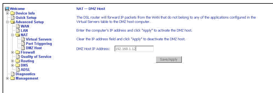
Figure 44: DMZ Host Setup
