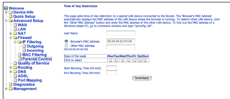
Figure 56: Parental Control – Time of Day Restrictions
