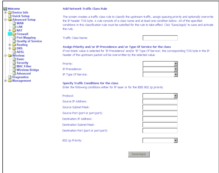
Figure 60: Quality of Service Add Screen
