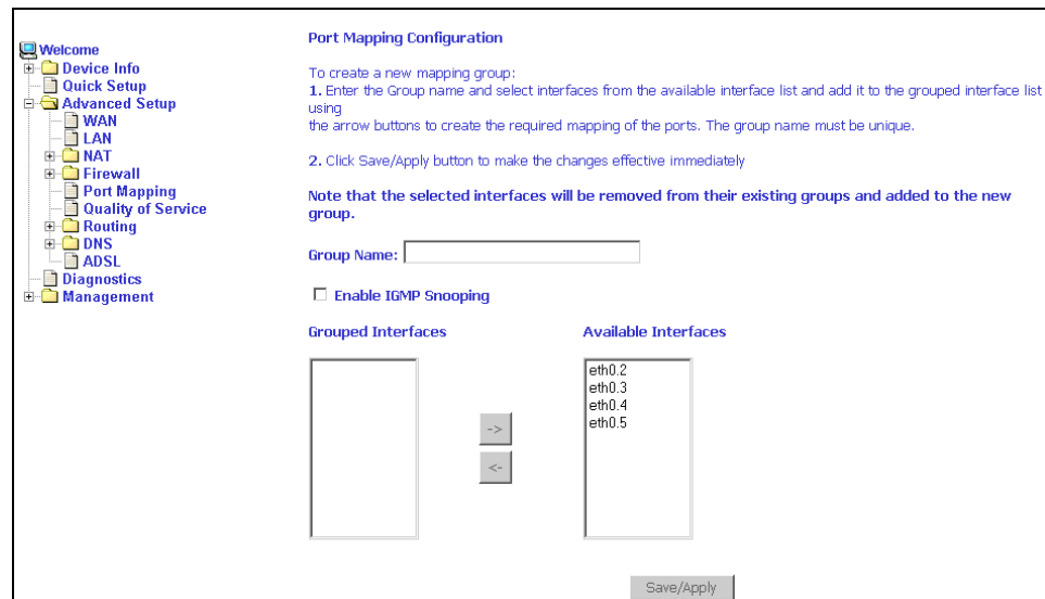
Figure 58: Creating a Port Mapping Entry
