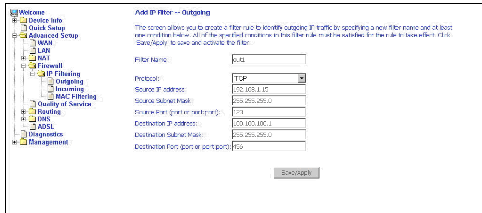
Figure 46: IP Filtering - Outgoing Filter Add Page
