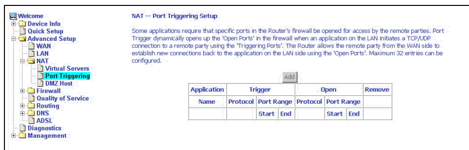
Figure 41: Port Triggering Setup Page
