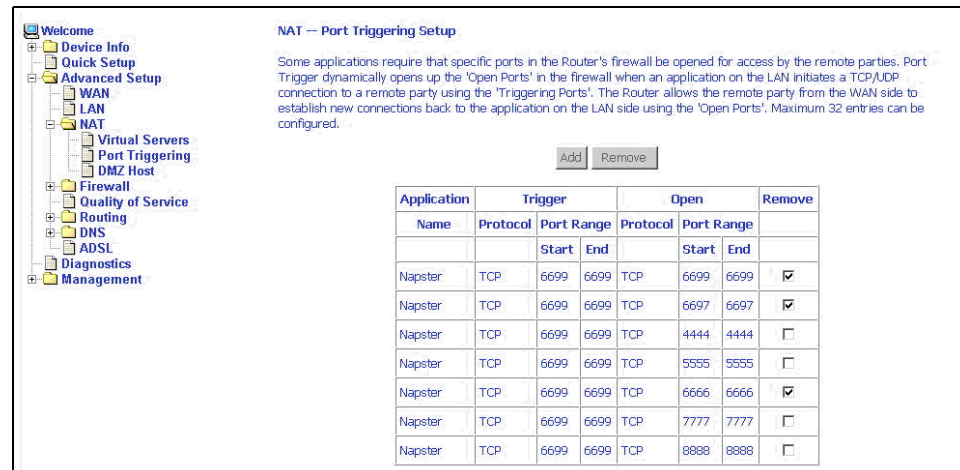
Figure 43: Port Triggering List
