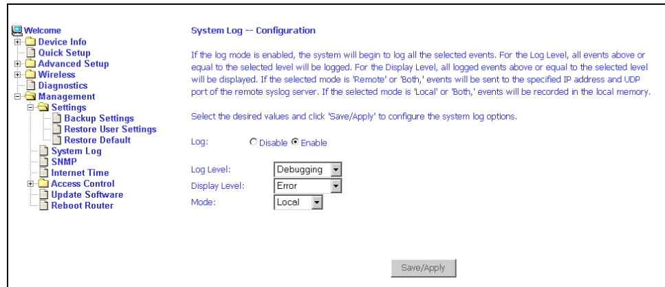
Figure 84: System Log Configuration
