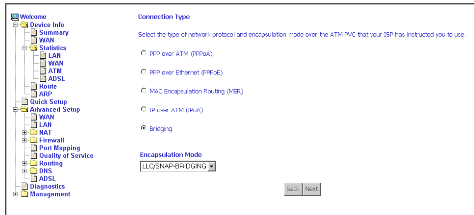
Figure 33: Connection Type Screen
