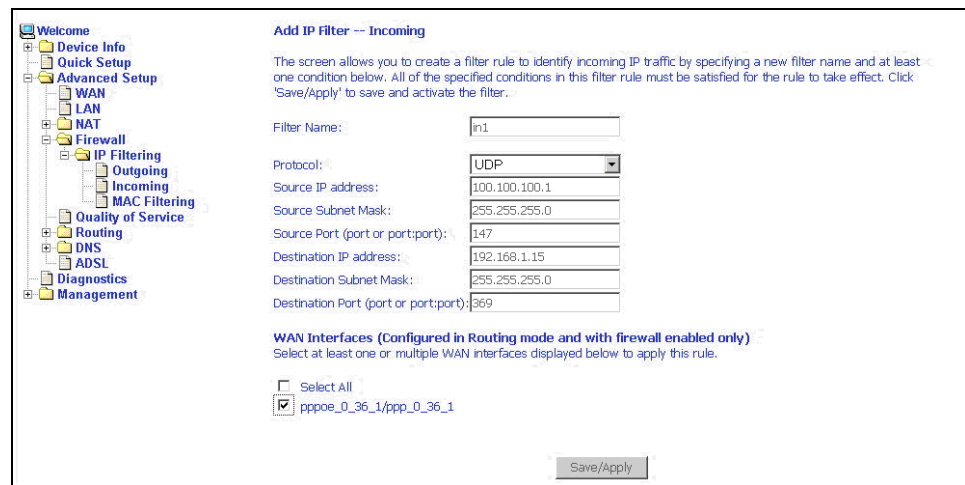
Figure 49: IP Filtering - Incoming Filter Add
