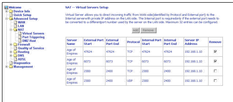
Figure 40: Removing Selected Virtual Servers
