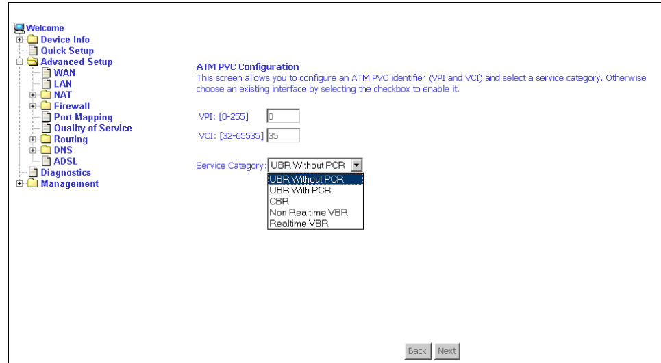
Figure 32: ATM PVC Configuration Screen
