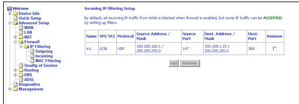
Figure 50: IP Filtering - Incoming Filtering List
