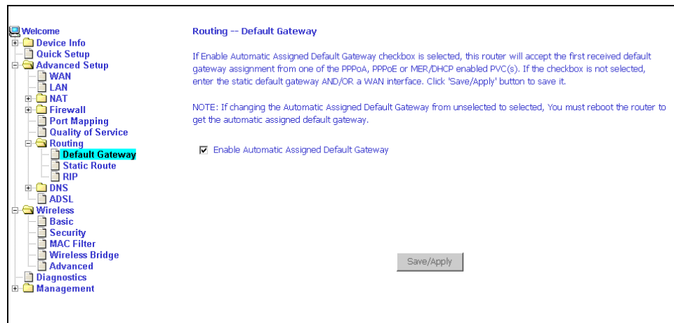
Figure 61: Default Gateway Setup
