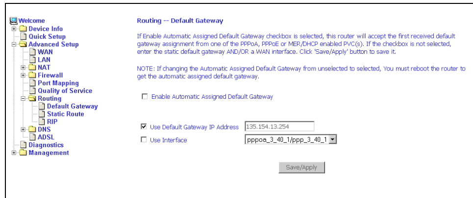
Figure 62: Default Gateway Setup
