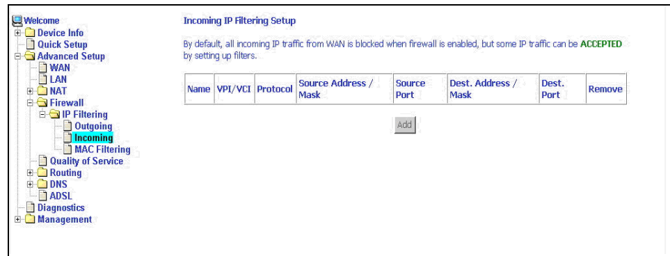
Figure 48: IP Filtering – Incoming Filter Setup Page
