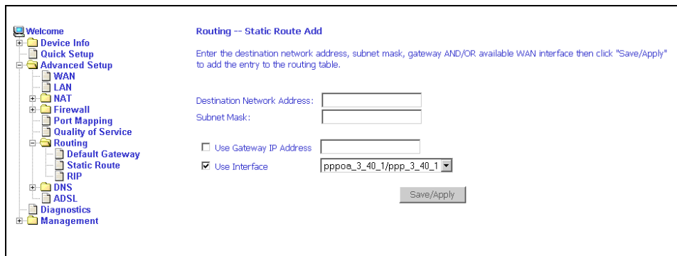
Figure 64: Static Route Add
