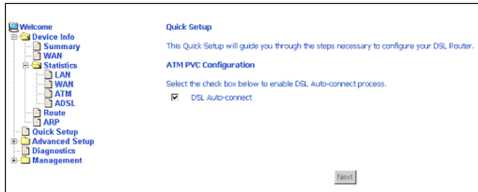
Figure 22: Quick Setup Initial Screen
