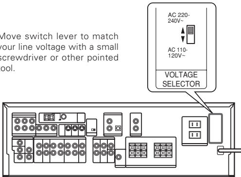
AC voltage selector switch
