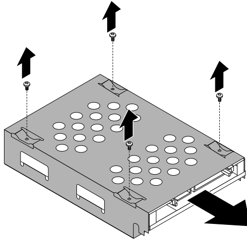
Figure 12. Removing the hard disk drive from the bracket
