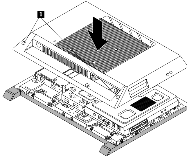
Figure 42. Installing the computer cover
