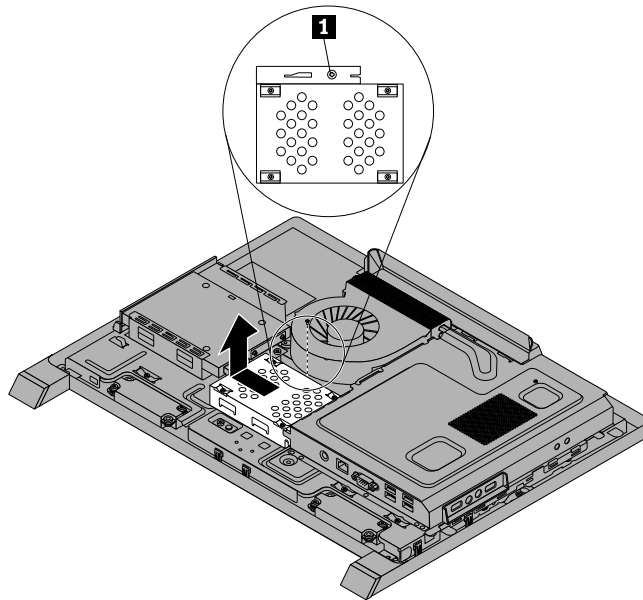
Figure 11. Removing the hard disk drive
