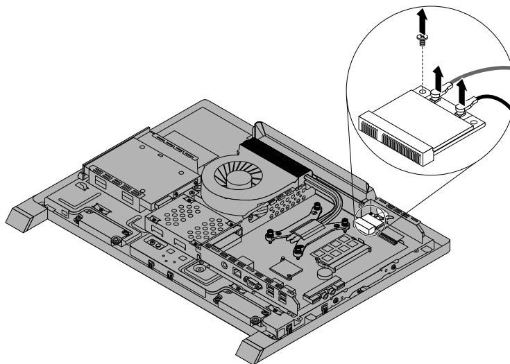
Figure 39. Removing the screw that secures the Wi-Fi card
