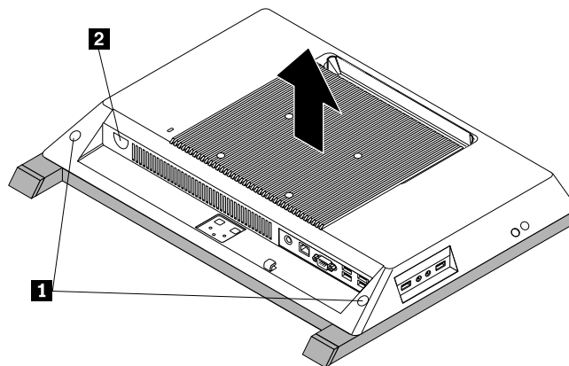
Figure 9. Removing the computer cover
