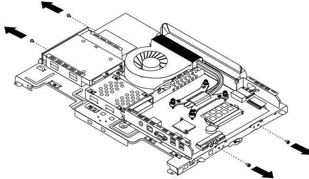
Figure 36. Removing the four screws that secure the LCD panel
