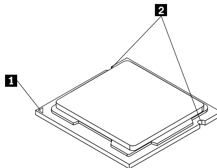
Figure 22. Noting the orientation of the microprocessor in the socket
