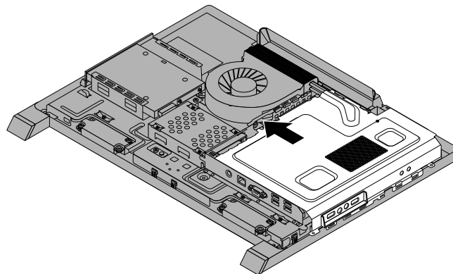
Figure 18. Installing the system board shield
