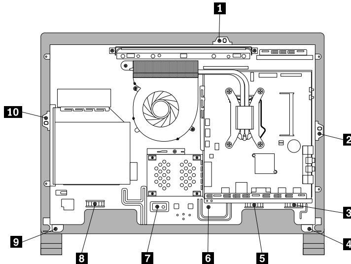
Figure 37. Reinstalling the 10 screws that secure the computer main bracket to the front bezel
