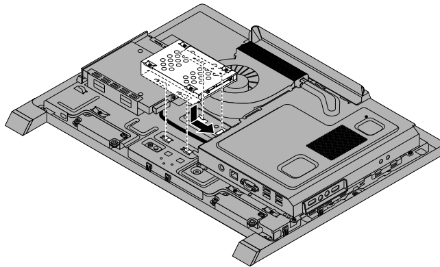
Figure 13. Installing the hard disk drive
