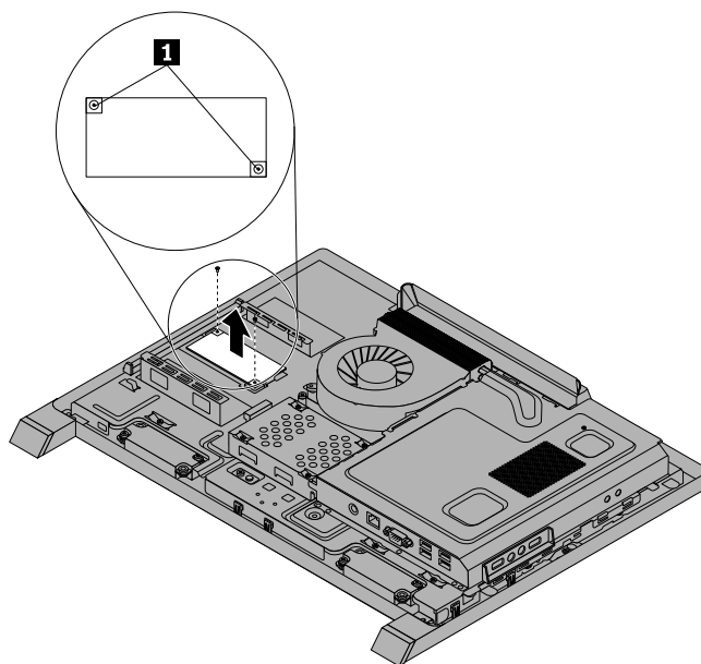
Figure 27. Removing the screws that secure the inverter
