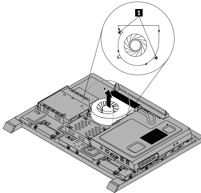
Figure 19. Removing the microprocessor fan
