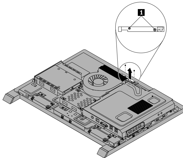
Figure 31. Removing the integrated camera
