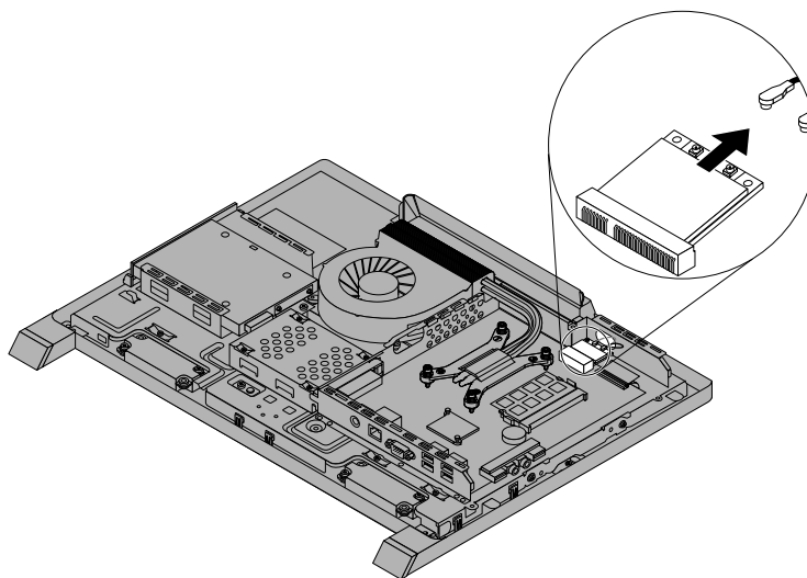
Figure 40. Removing the Wi-Fi card
