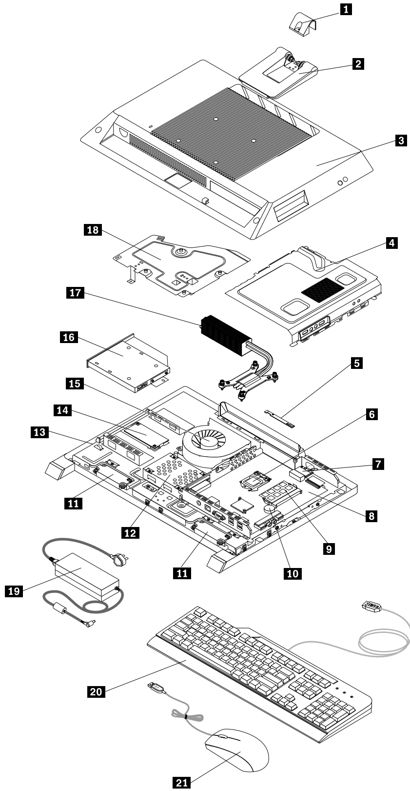
Figure 3. Locating major FRUs and CRUs
