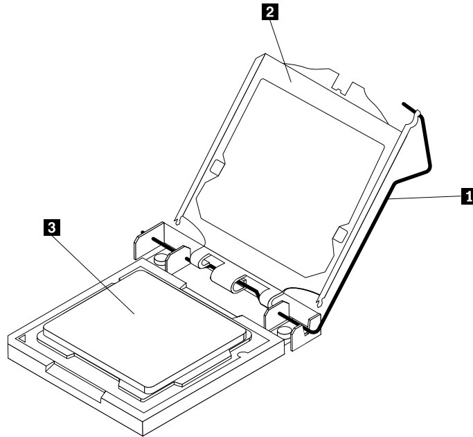
Figure 21. Opening the retainer to access the microprocessor
