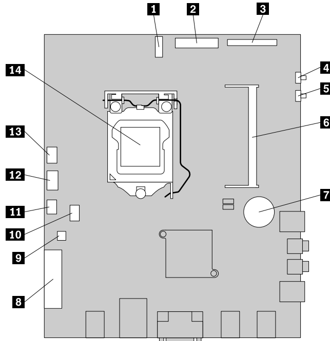
Figure 4. Locations of the parts and connectors on the system board
