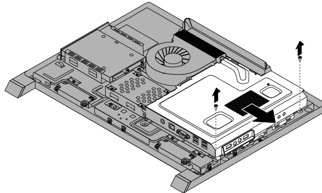
Figure 17. Removing the system board shield
