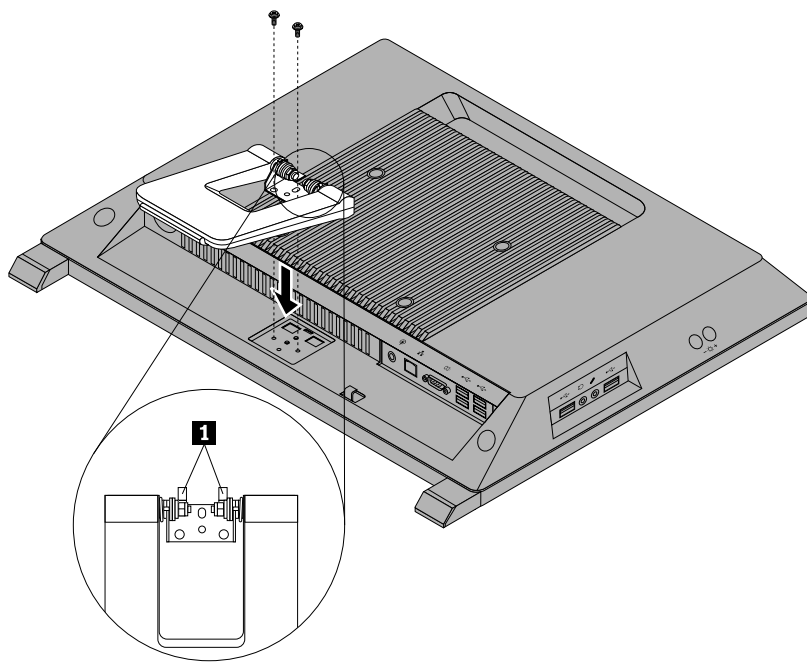
Figure 8. Reinstalling the system stand
