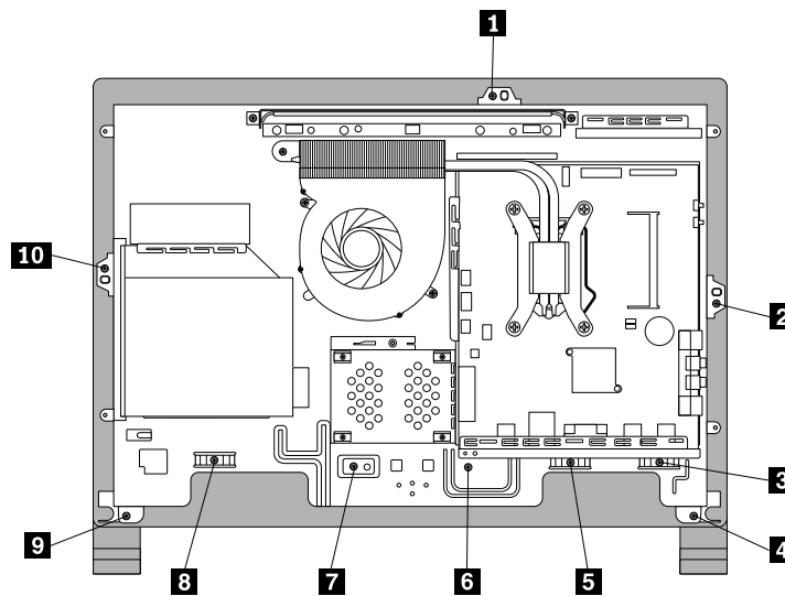
Figure 35. Removing the 10 screws that secure the computer main bracket to the front bezel
