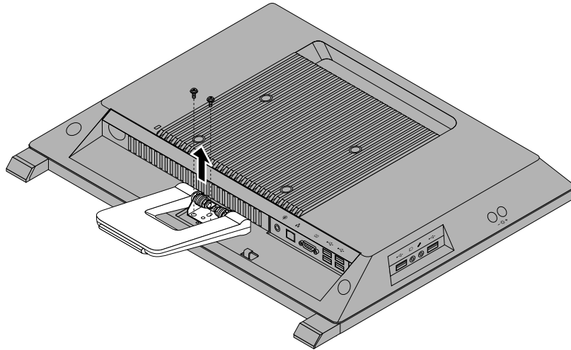
Figure 7. Removing the system stand
