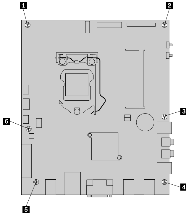
Figure 32. Removing the six screws that secure the system board to the main bracket
