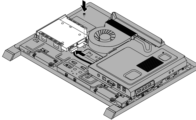
Figure 16. Connecting the cable and installing the screw
