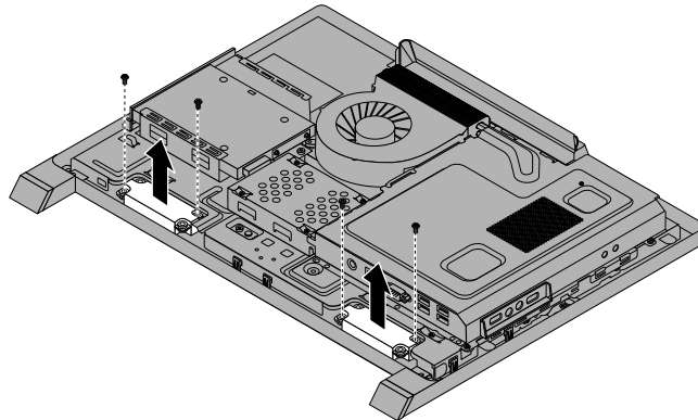
Figure 30. Removing the internal speakers
