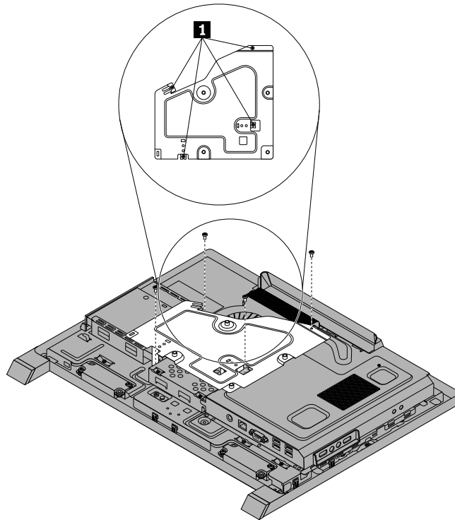
Figure 10. Removing the VESA mount bracket
