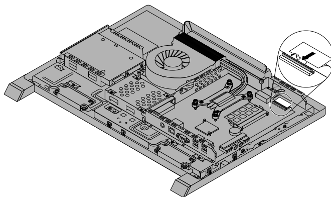
Figure 38. Reconnect the LCD panel cable to the system board
