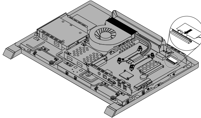
Figure 34. Disconnect the LCD panel cable from the system board
